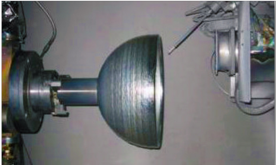
Figure 4: Additively Manufacturing a Satellite Propellant Tank Using Electron Beam Technology
