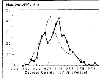
Figure 6. Histogram showing actual data (N = 367) from satellites over the period (December 1978 to June 2009). Each solid square represents the number of months that the temperature of the troposphere (above the southern hemisphere oceans) varied from an arbitrary mean value. Data (ie. solid squares) obtained from the Climate Center University of Alabama at Huntsville ( http://www.ncdc.noaa.gov/oa/climate/research/uahncdc.lt ). The dashed line represents a hypothetical distribution from a cooler period in the past. In this graph, the tails from both curves are deliberately identical. The hypothetical line was drawn so that the probability of extreme events is not changed.
