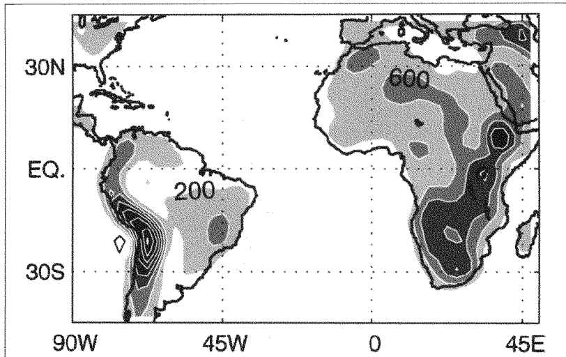
Figure 4: Representation of topography using a standard T42 truncation scheme in a spectrally-based climate model. The contour interval is 400 m. Negative altitudes of below -200 m occur west of the Andes while the highest peaks are only 3000 m high. Note also the inaccuracies of the representation of topography in Africa (from Biasutti et al. , 2003).
