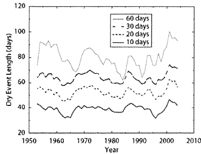
Figure 7. Five year moving average time series of mean dry event length (computed using minimum dry event lengths of 10, 20, 30, and 60 days) for warm seasons (April through September).
