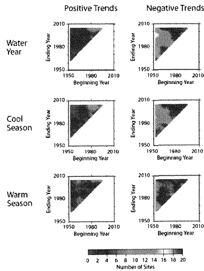
Figure 8. Number of sites with statistically significant (at a 95% confidence level ( p = 0.05 )) positive and negative trends in 5 year moving average time series of mean dry event length (using dry events with a minimum length of 10 days) for water years and cool and warm seasons. The beginning and ending dates refer to the center year of the 5 year moving period. The statistical significance of trends was determined using Kendall's tau.
