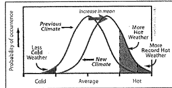
Figure 5. Schematic showing the IPCC view that little or no skew and kurtosis occurs when the mode shifts by +0.7°C. The authors suggest the probability of extreme low temperatures decrease in proportion to the probability of high temperature (Figure 1, Box TS.5 from IPCC 2007a).
