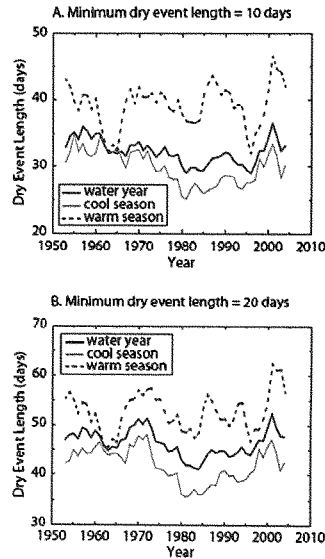
Figure 6. Five year moving average time series of mean dry event length (computed using minimum dry event lengths of 10 and 20 days) for water years (October through September), cool seasons (October through March), and warm seasons (April through September).
