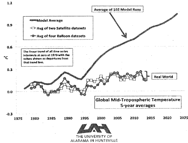
Figure 1. Model projections of global mid-tropospheric temperature (red line) compared to observed temperatures (blue and green lines). Figure courtesy of Dr. John Christy
