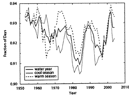
Figure 4. Five year moving time series of the mean fraction of days with daily precipitation below 2.54 mm for water years (October through September), cool seasons (October through March), and warm seasons (April through September).
