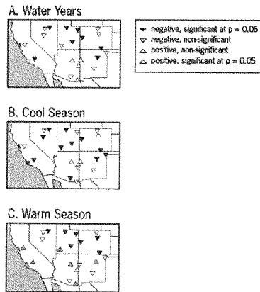
Figure 3. Trends in 5 year moving fraction of days with daily precipitation below 2.54 mm, from 1951 to 2006. The statistical significance of trends (at a 95% confidence level ( p = 0.05 )) was determined using Kendall's tau.
