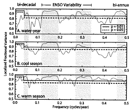
Figure 9. Localized fractional variance spectrum from a spectral analysis of 5 year moving average fraction of dry days for 22 sites in the southwestern United States for the period 1951 through 2006 (gray line). The horizontal lines indicate the 95% ( p = 0.05 ) and 99% ( p = 0.01 ) confidence levels. The gray shaded bars indicate statistically significant frequencies (at p < 0.05 ) that are common among water years and cool and warm seasons.
