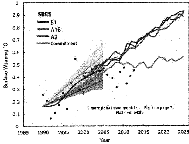
Figure 1. Model projections of global temperature change compared to observed (HadCRUT3) surface temperature means (Solid dots). Observations since 2005 have been lower than projected. Adapted from Figure TS.26 in IPCC technical summary http://tinyurl.com/7gjkvzf .
