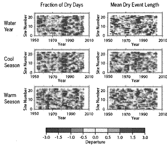
Figure 2. Time series of standardized departures of the fraction of dry days and dry event length for each site and for water years, cool seasons, and warm seasons. Site numbers correspond to the site numbers in Figure 1 and Table 1.
