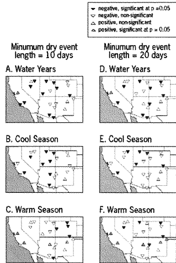
Figure 5. Trends in the 5 year moving mean length of dry events (computed using a minimum dry event length of 10 and 20 days) for water years (October through September), cool seasons (October through March), and warm seasons (April through September). The statistical significance of trends (at a 95% confidence level ( p = 0.05 )) was determined using Kendall's tau.
