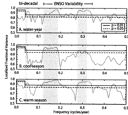
Figure 10. Localized fractional variance spectrum from a spectral analysis of 5 year moving average dry event lengths for 22 sites in the southwestern United States for the period 1951 through 2006 (gray line). The horizontal lines indicate the 95% ( p = 0.05 ) and 99% ( p = 0.01 ) confidence levels. The gray shaded bars indicate statistically significant frequencies (at p < 0.05 ) that are common among water years and cool and warm seasons.
