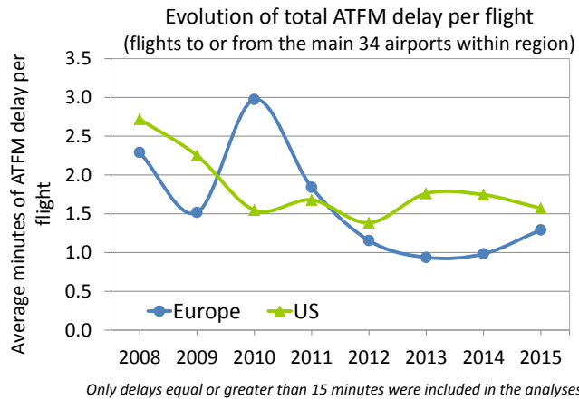
Figure 5-2: Evolution of total ATFM delay per flight (2008-2015)
