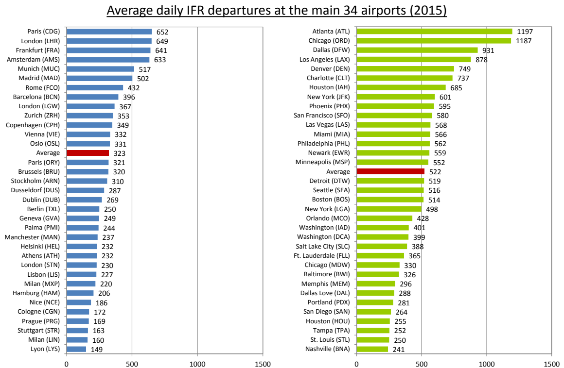
Figure 3-8: Operations at the main 34 airports (2015)
