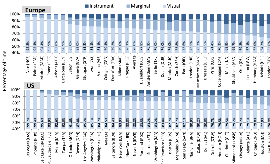
Figure 3-15: Percent of time by meteorological condition at the main 34 airports (2015)
