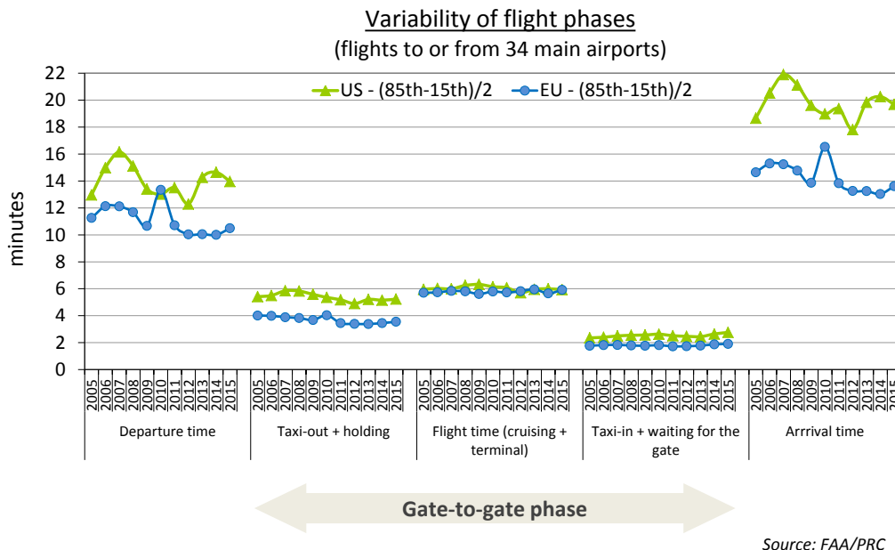
Figure 4-8: Variability of flight phases (2005-2015)
