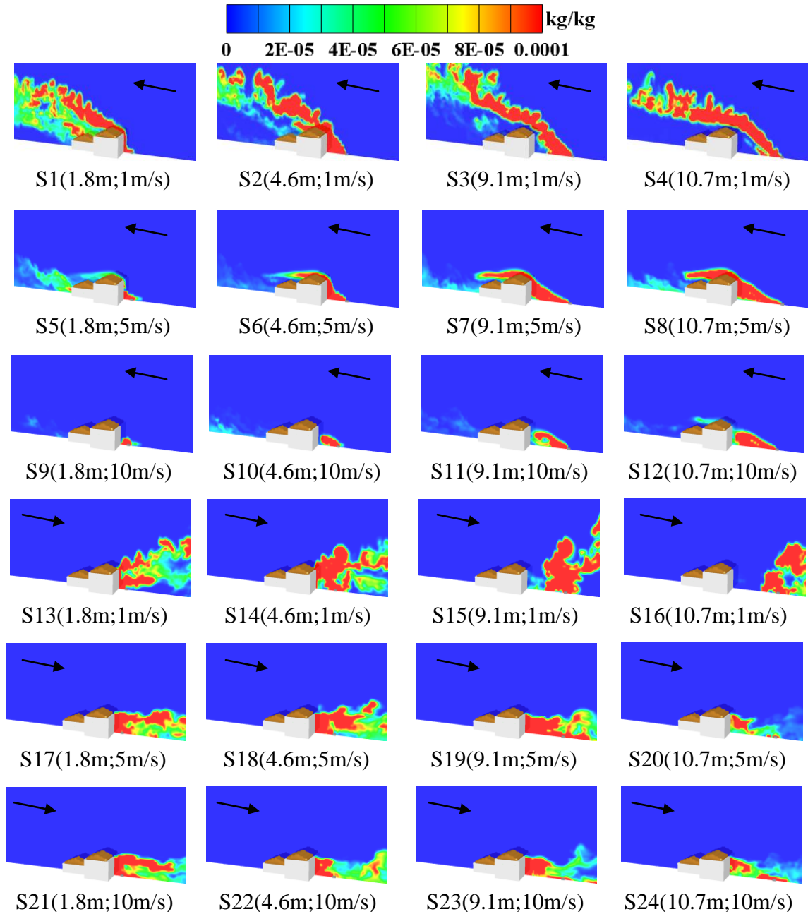
Figure 4. Comparison of CO levels at the middle lengthwise plane of the house for different generator distance, location, wind direction and speed when the generator exhaust pointed towards the house.
