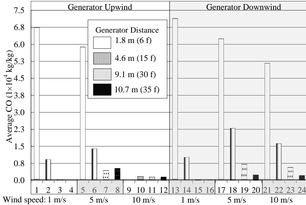
Figure 6. Comparison of time-average CO levels for all windows, doors and other leaks at the house envelope when the generator exhaust pointed towards the house (for CO in air, 1.0 kg/kg \approx 1.2 \times 10^6 mg/m 3 at 20.9 °C and 101.325 kPa).
