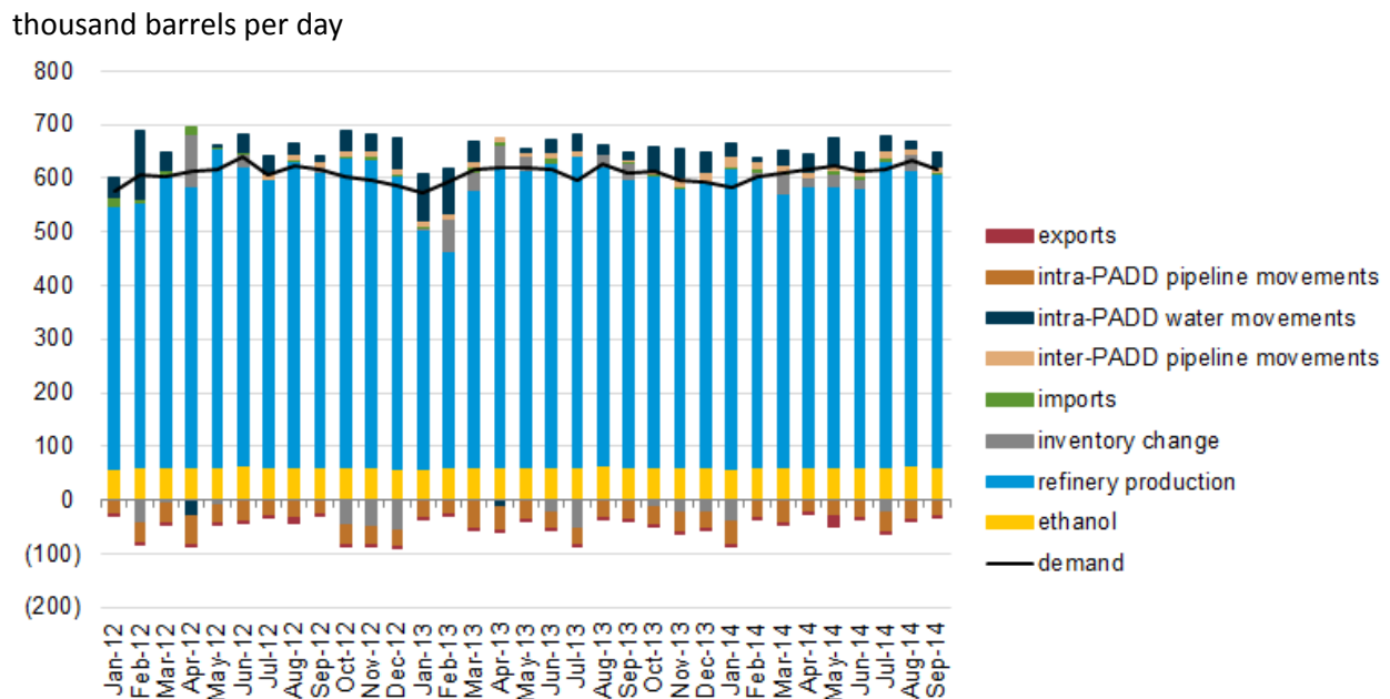
Figure 10. Southern California and Southern Nevada motor gasoline supply/demand balance
