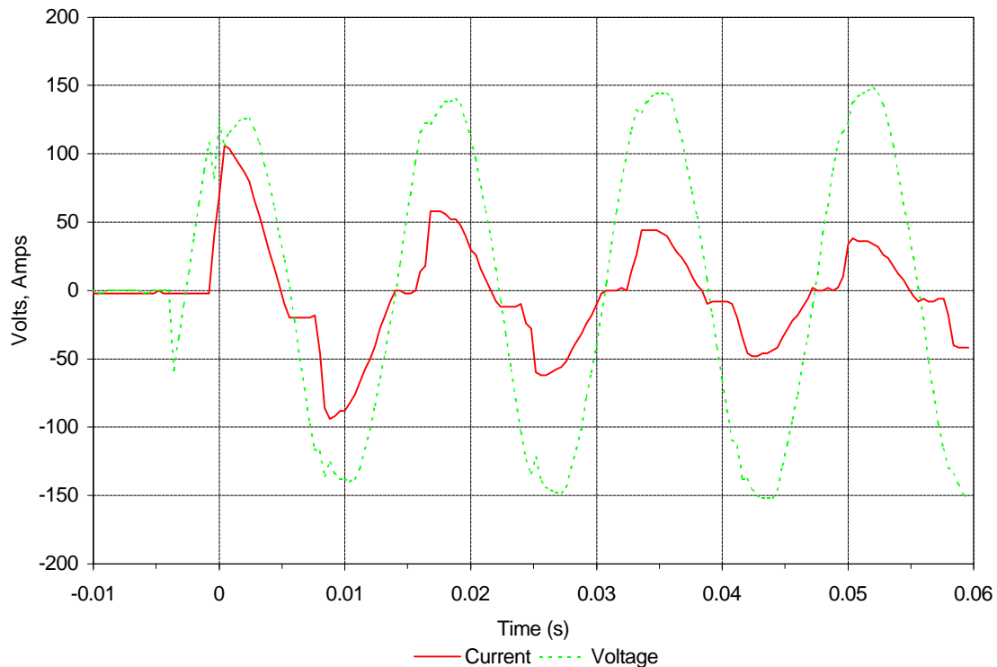
(3) 500 Watt Halogen Lamps Voltage and Current
