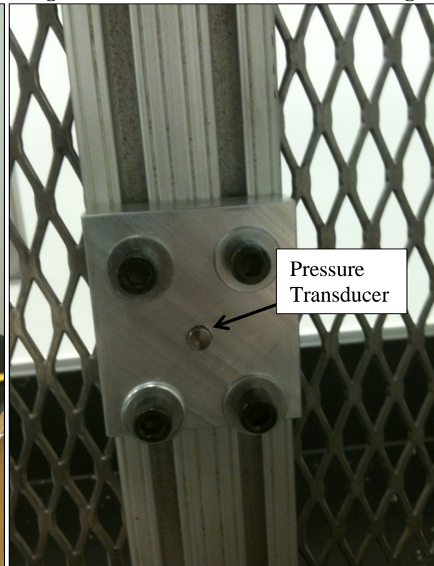
Figure 3: Pressure Transducer Mounting
