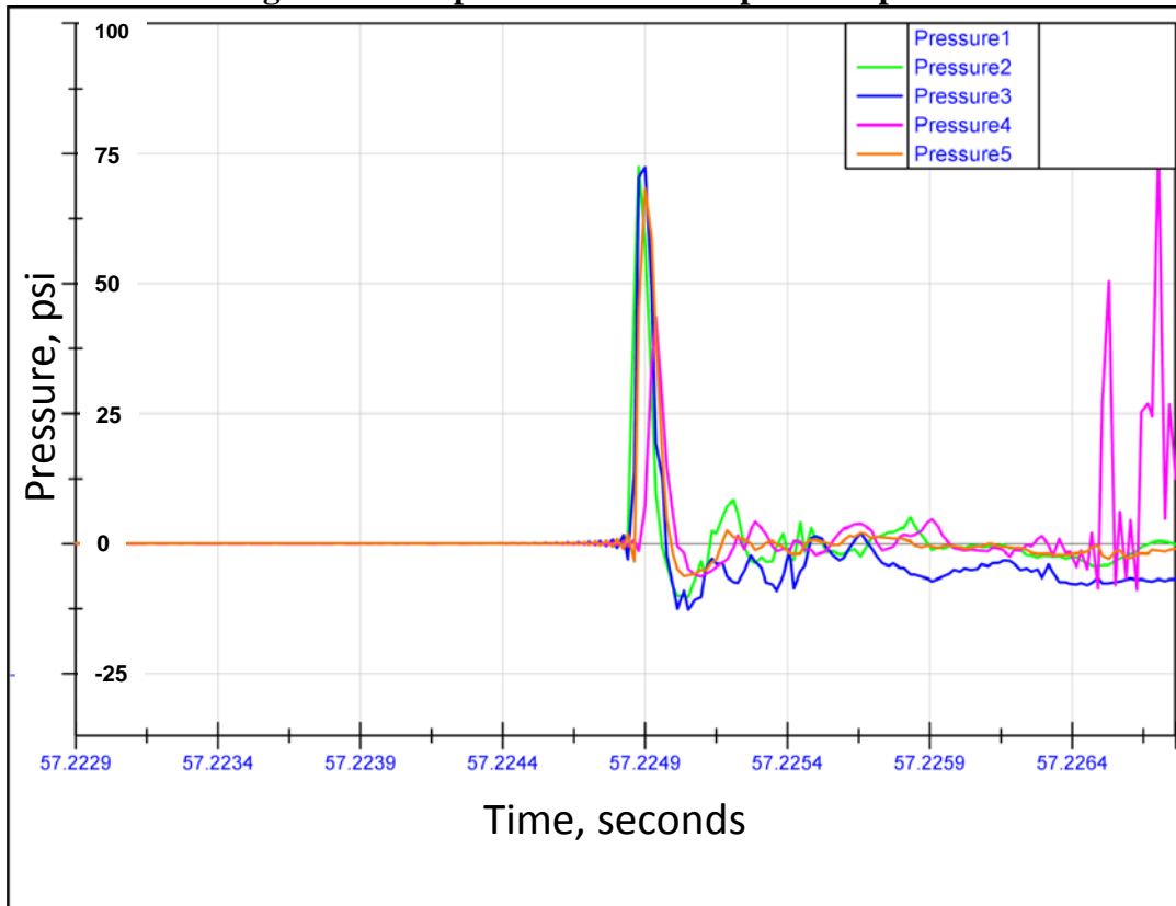
Figure 5: Overpressure from Sample w/ Report
