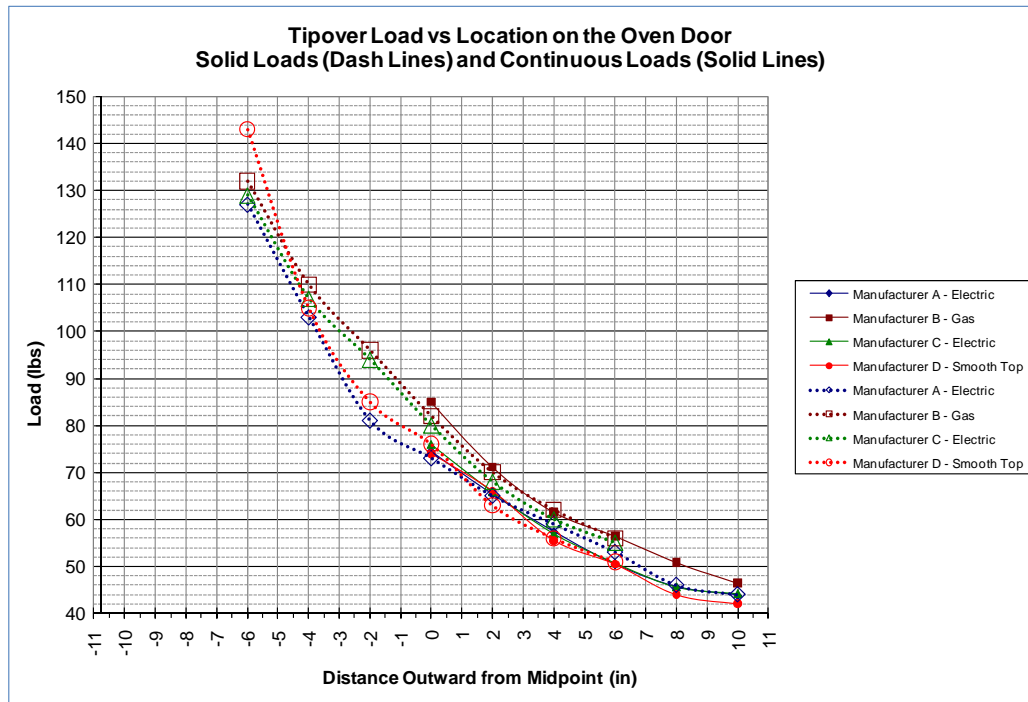
Figure 3. Tipover Forces
