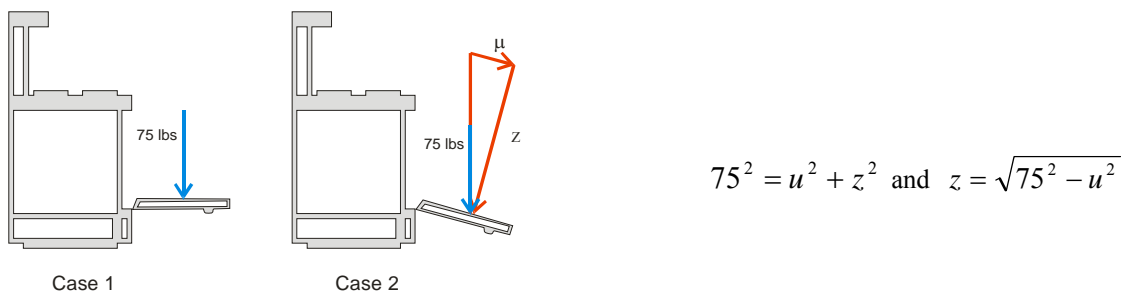
Figure 6. Force to Tip a Sagging Oven Door
