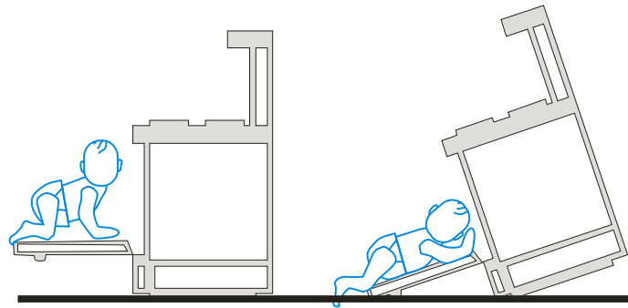
Before Range Tips Forward After Range Tips Forward Figure 50. Illustration of Oven Door Locking in the Open Position After Tipover
