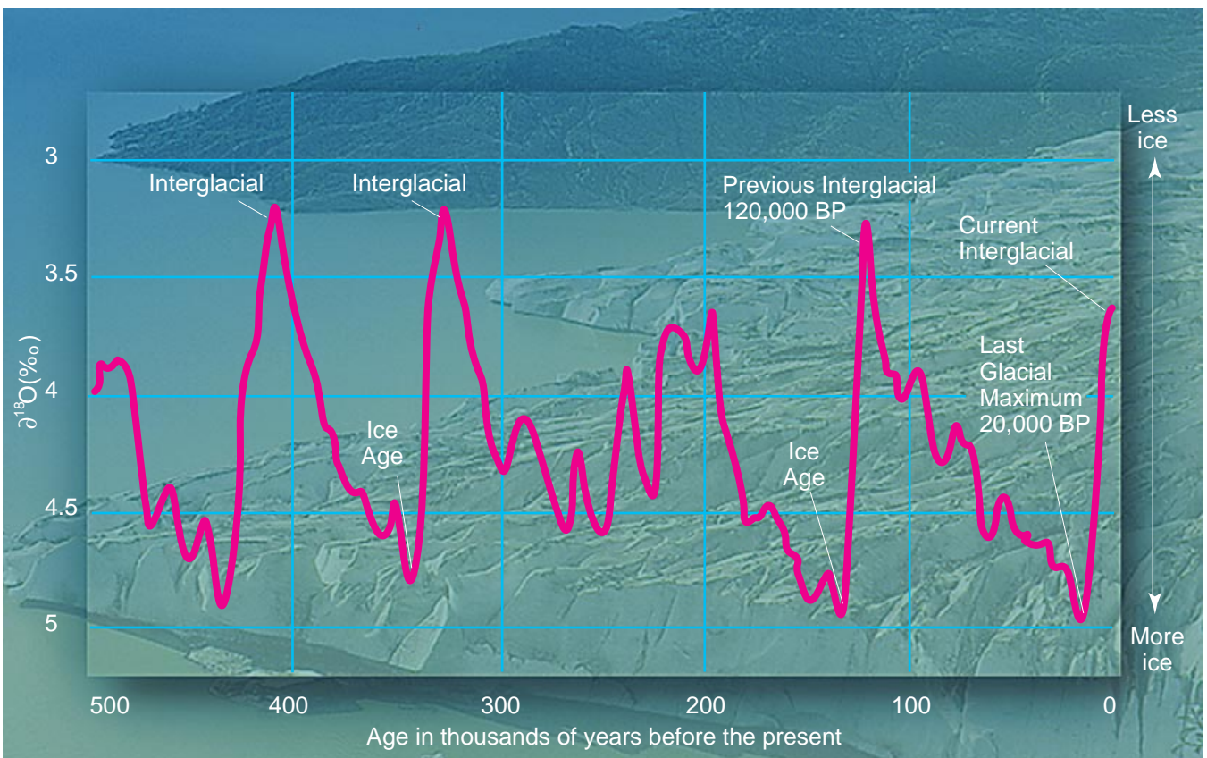
Oxygen Isotope—Global Ice Volume Past 500,000 Years
