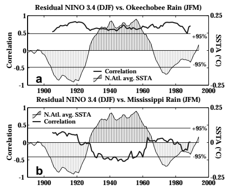
Figure 3. (a) Ten-year running DJF mean of the AMO index (shaded departures) shown in comparison with the 20-year running correlation between the NINO-3.4 SSTA index for Dec.-Feb. and the unsmoothed Jan.-Mar. rainfall anomaly of Florida climate division 4 (heavy, solid). (b) As above, but for the area-weighted rainfall accumulation over the Mississippi basin.
