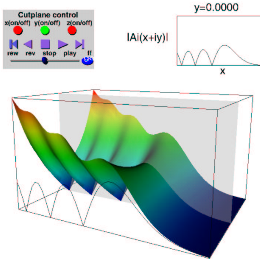
Figure 5. View of the Airy function z = |Ai(x+iy)| . The surface in xyz -coordinates is cut by the xz -plane to display oscillatory behavior along the negative real axis. The zeros, to 2 decimals, are -2.34, -4.09, -5.52 . Exponential growth and decay in different parts of the complex plane are visible also. ©National Institute of Standards and Technology.
