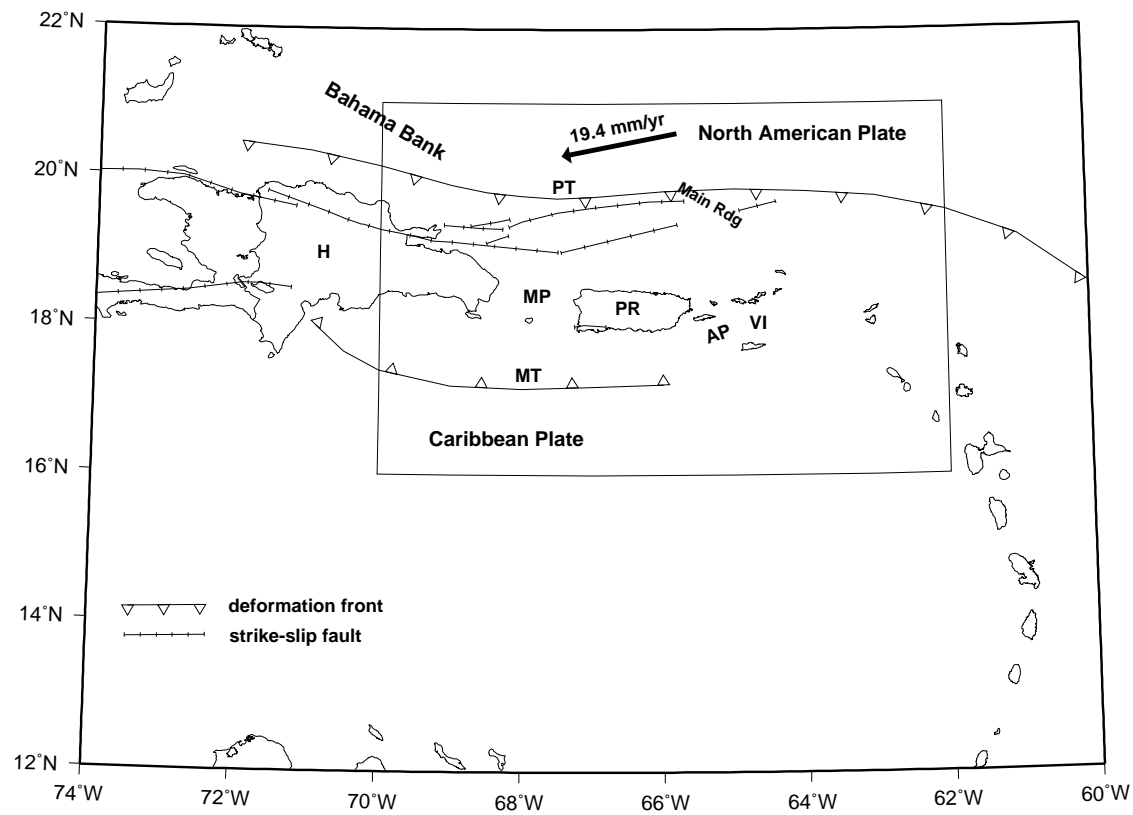
Fig.1: Map of North American - Caribbean plate boundary region. Inset box shows area of seismic hazard analysis. Arrow shows motion of North American plate relative to Caribbean plate from Jansma et al. (2000). Structural elements generalized from Grindlay et al. (1997), Dolan et al. (1998), and LaForge and McCann (2003). Abbreviations: H= Hispaniola, PR= Puerto Rico, VI= Virgin Islands, PT= Puerto Rico Trench, MT= Muertos Trough, MP= Mona Passage, AP= Aneгада Passage.
