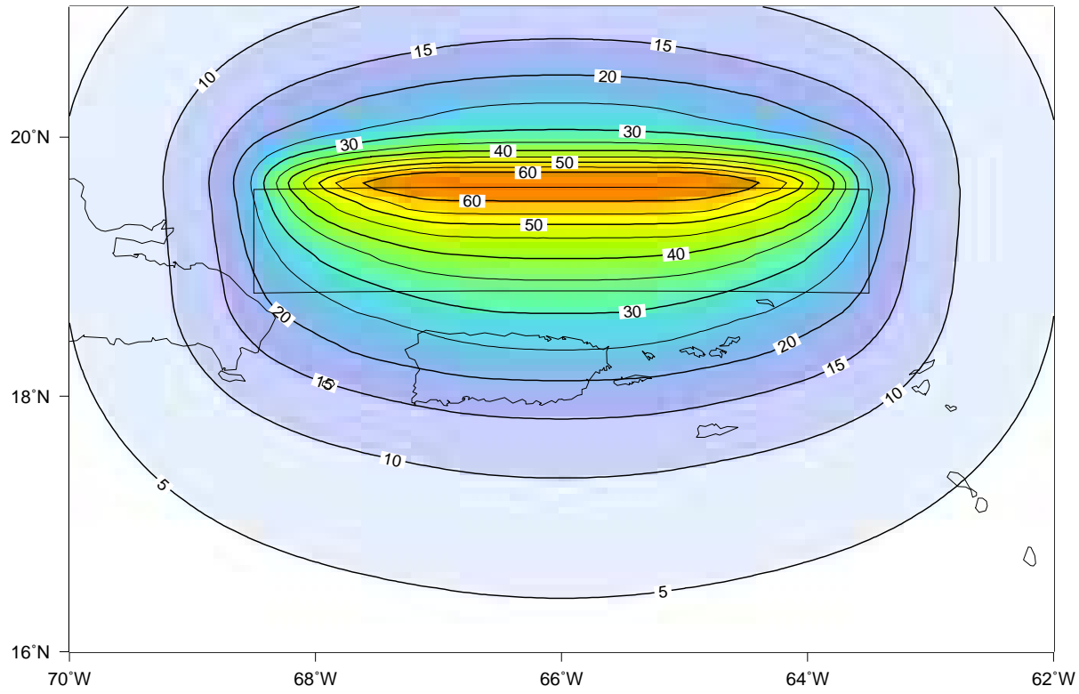
Fig.3c: PGA (%g) with 2% probability of exceedance in 50 years from Puerto Rico subduction.
