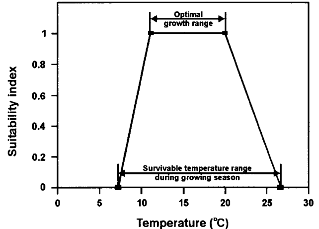
Fig. 4-39. Temperature suitability index curve constructed by overlaying two sets of binary criteria for growth and survival. The suitability index is a sliding scale wherein a score of 1.0 represents the optimum temperature range and 0.0 indicates unsuitable temperatures.
