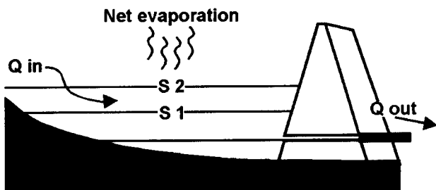
Fig. 5-8. Components of a reservoir mass balance model. S1 represents the volume in the reservoir at time (t) and S2 is the storage goal from the rule curve at time (t + 1) . Q in is inflow and Q out is outflow.
