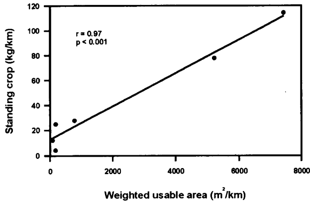
Fig. 4-25. Relation between weighted usable area and standing crop of cutthroat trout ( Oncorhynchus clarkii ) for six sites in Yellowstone National Park.
