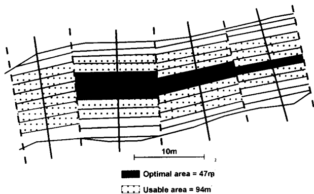
Fig. 4-15. PHABSIM's translation of the distribution of structural and hydraulic characteristics into an area of suitable microhabitat for a target species.
