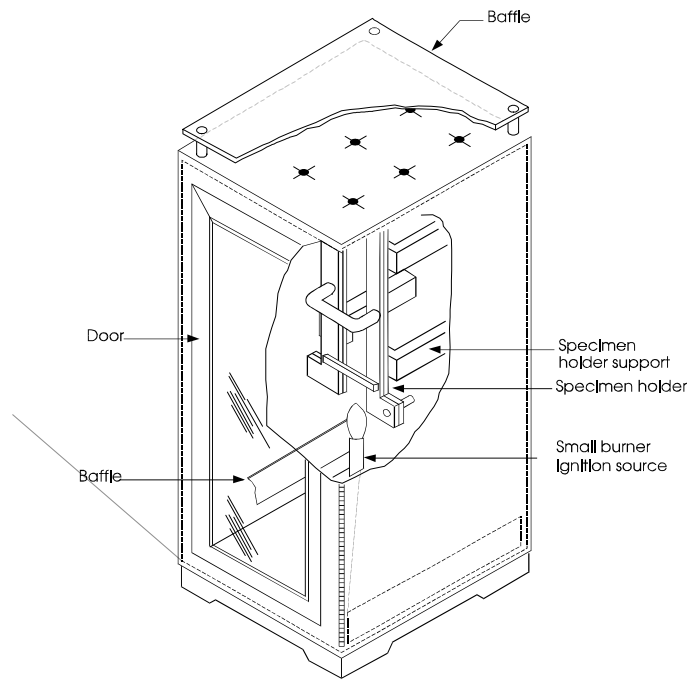
Figure B-4. FAR 25.853 (a) Test Apparatus
