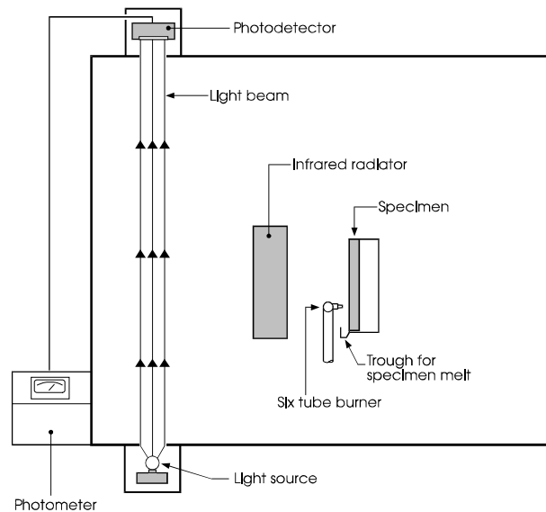
Figure B-2. ASTM E 662 Test Apparatus
