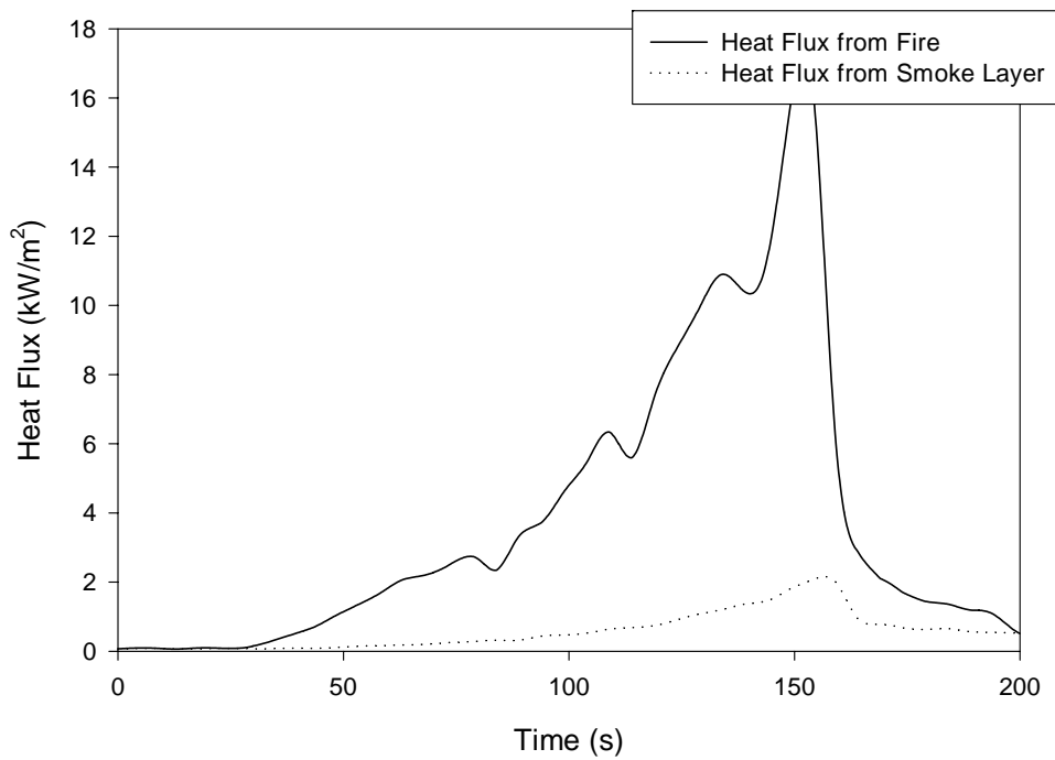
Figure B-39. Test 5 (Medium Gas Burner), Heat Flux Data
