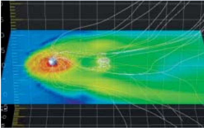
Modeling reconnection in the magnetotail.
