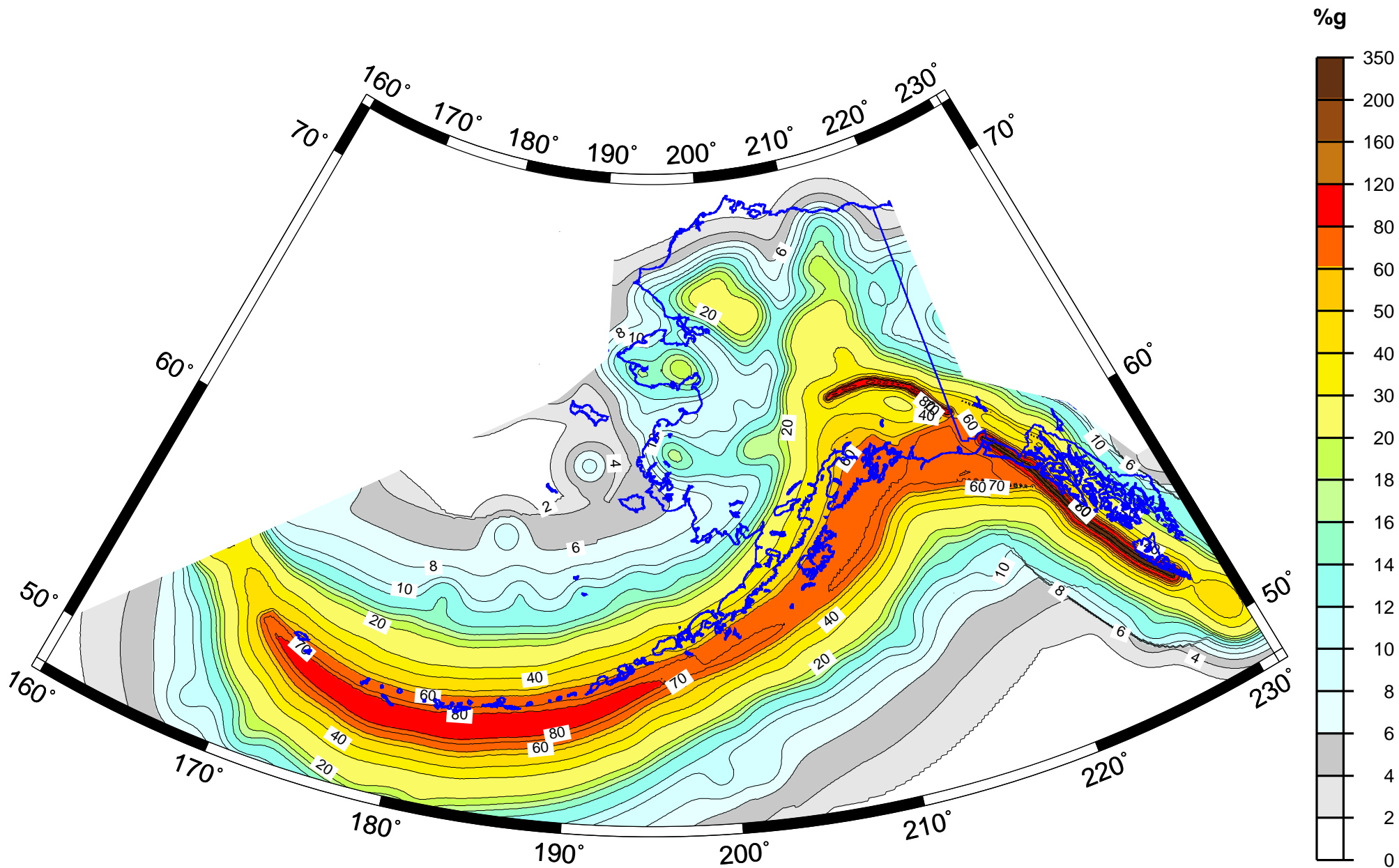
1 Hz Spectral Acceleration (%g) with 2% Probability of Exceedance in 50 Years
