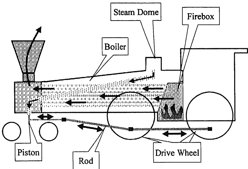
Figure 3 Major components of a steam locomotive.
