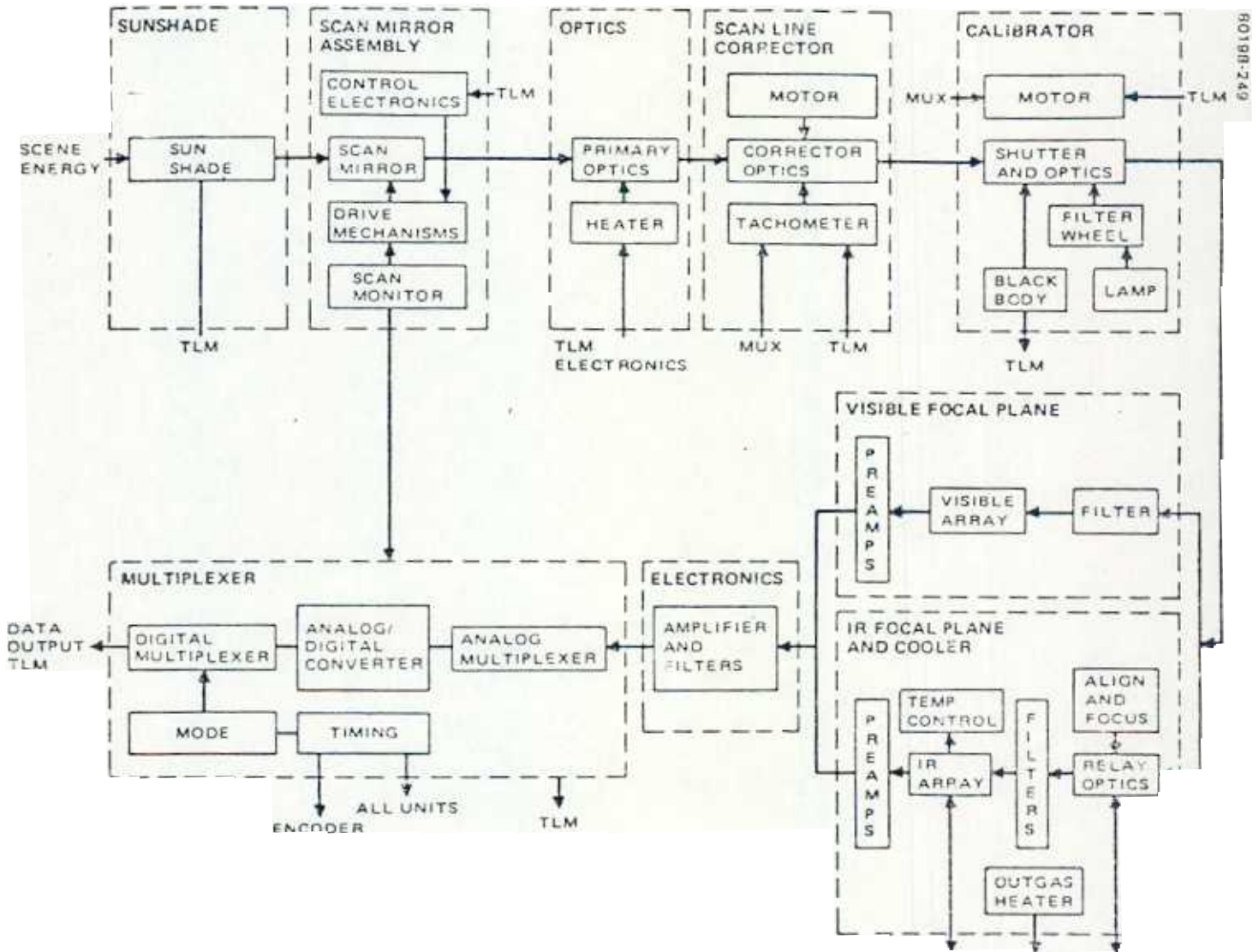
Figure 1-5. Thematic Mapper Functional Block Diagram
