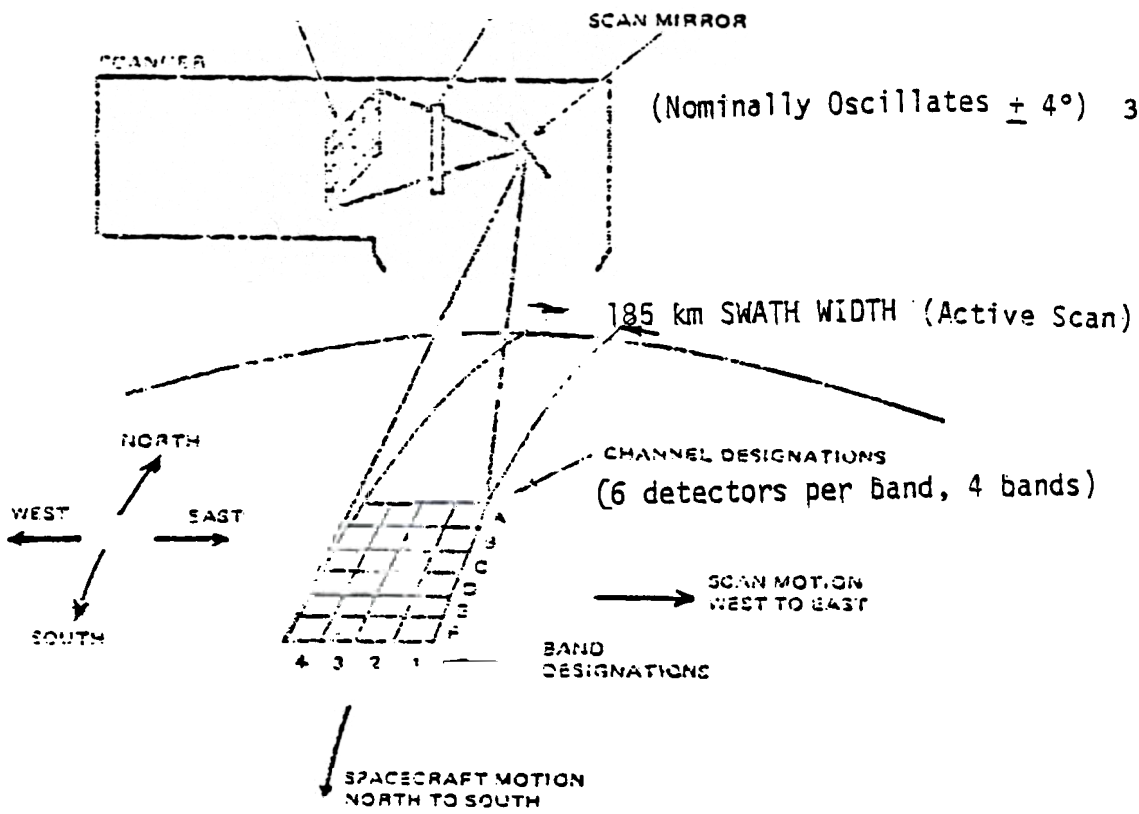
Figure 1-13. MSS Field Stop Pattern Projected on the Earth's Surface
