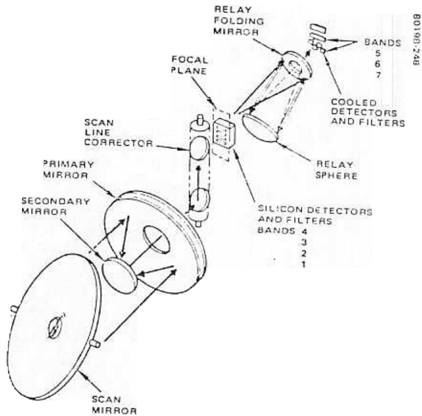
Figure 1-4. Thematic Mapper Optical System
