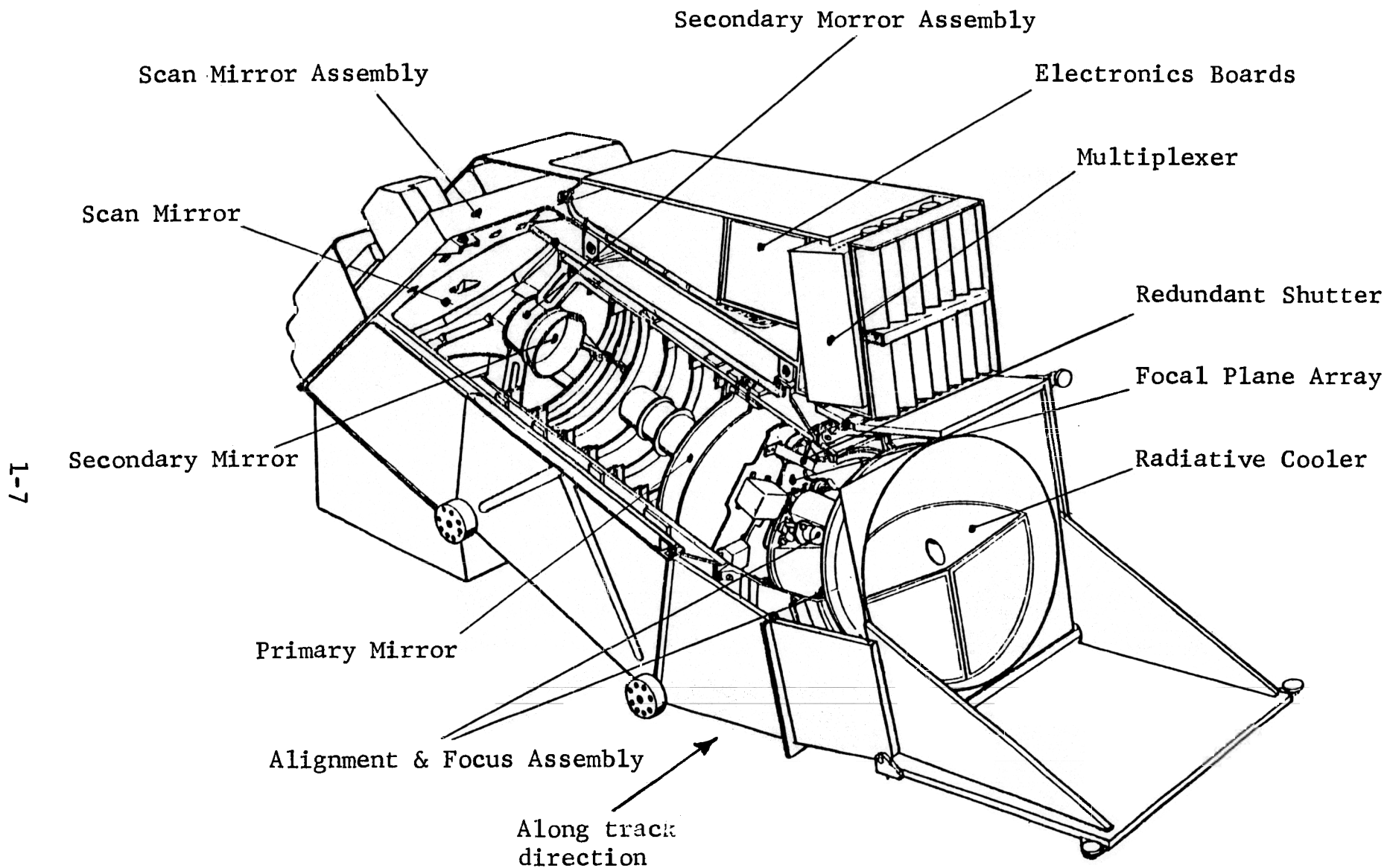
Figure 1 - 3 Thematic Mapper General Configuration
