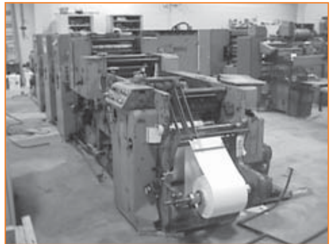
Figure 31. Roll-to-Roll Offset Printing Press
