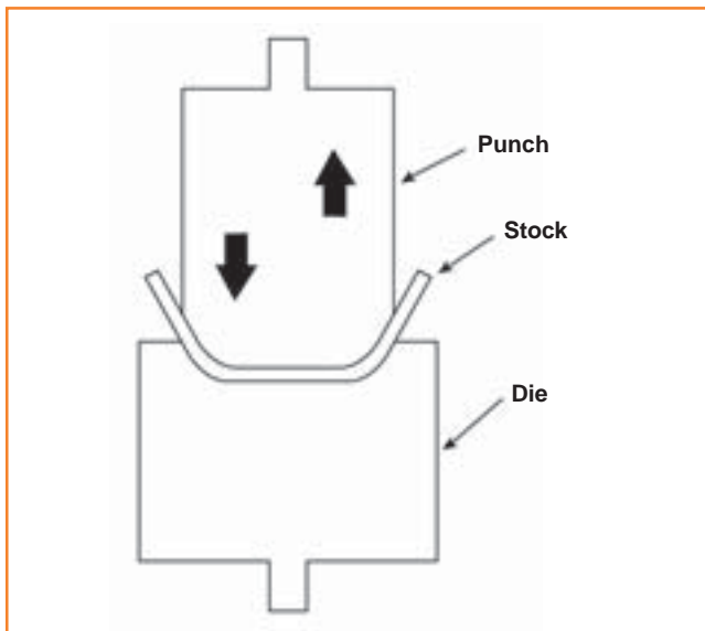
Figure 7. Bending Action
