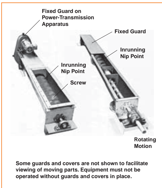
Figure 28. Screw Conveyor
