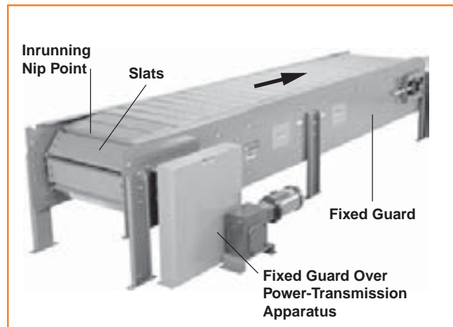
Figure 30. Slat Conveyor
