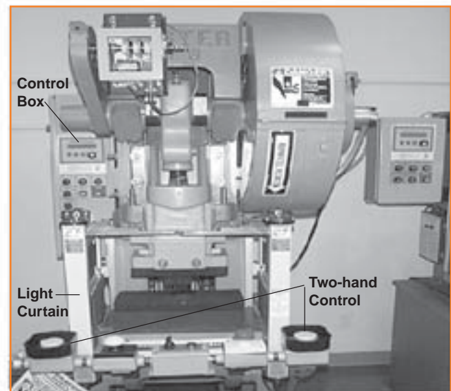
Figure 23. Part Revolution Mechanical Power Press with Two-Hand Control
