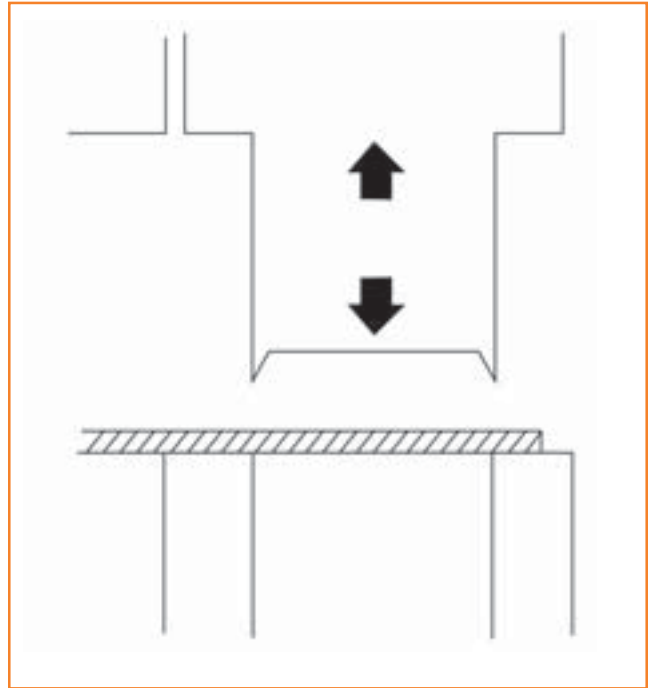
Figure 5. Punching Action
