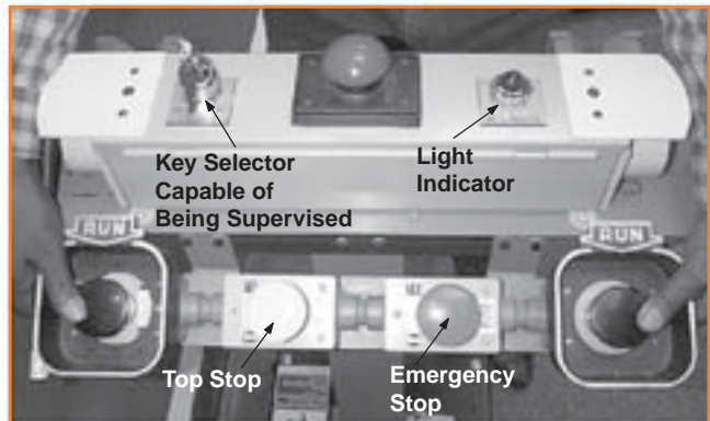
Figure 17. Two-Hand Control
