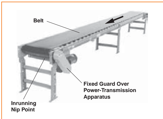
Figure 27. Belt Conveyor
