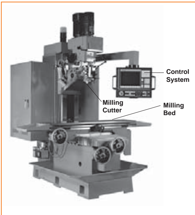
Figure 41. Bed Mill
