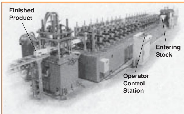
Figure 33. Roll-Forming Machine
