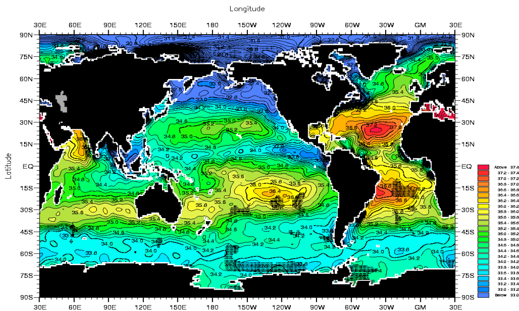
Fig. E2-1. Fall (Oct.-Dec.) mean salinity (PSS) at the surface. Minimum Value= 3.52 Maximum Value= 40.77 Contour Interval: 0.20
