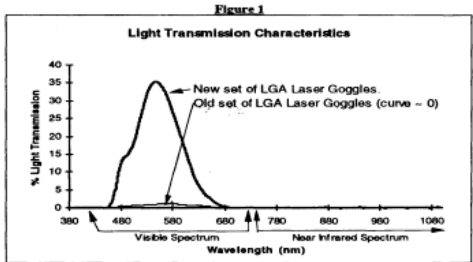
Figure 1: Comparison of Light Transmission characteristics of an older and a newer set of type-LGA laser eye protection goggles.
