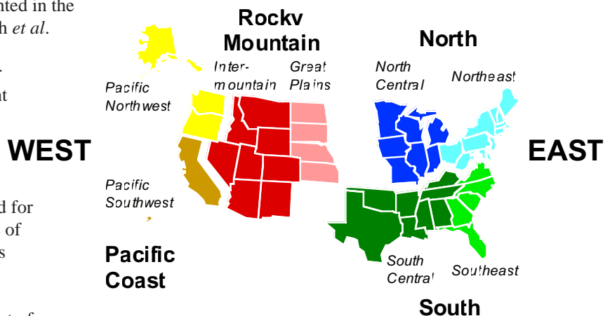
Figure 2 — Forest resource reporting regions and subregions of the United States.
