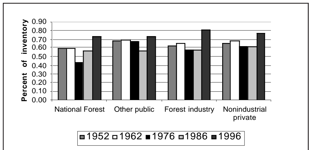
Figure 10 — Mortality as a percent of growing-stock volume on timberland by owner group, 1997.
