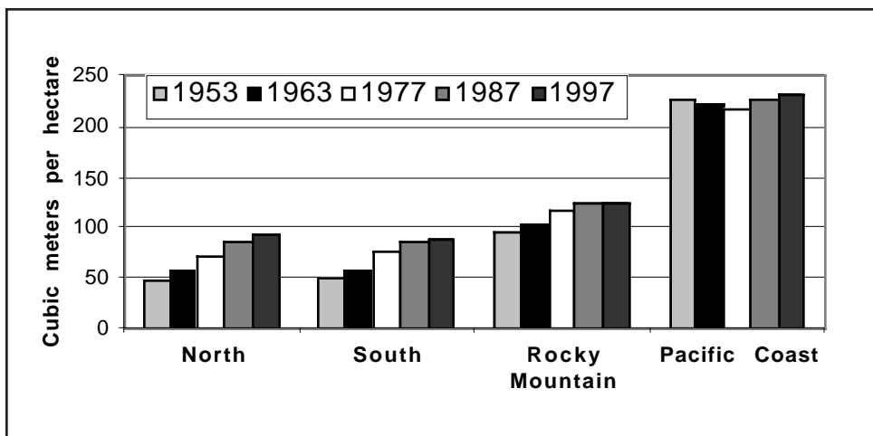
Figure 7 — Trends in average volume per hectare on timberland by region.
