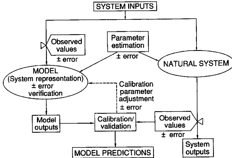
Fig. 5.1. Calibration process.
