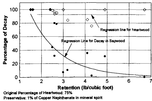
Fig. 4—Percentage of decay in heartwood and sapwood of southern pine after 32 years of field test (Huffman 1996)
