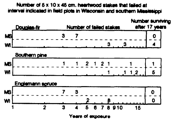
Fig. 2—Natural durability of Douglas-fir, southern pine, and Englemann spruce in Mississippi and Wisconsin.
