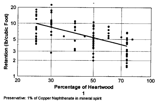
Fig. 1—Relation between amount of heartwood and retention in southern pine (Huffman 1996).
