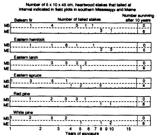
Fig. 3—Natural durability heartwood of the indicated softwood species in Mississippi and Maine.
