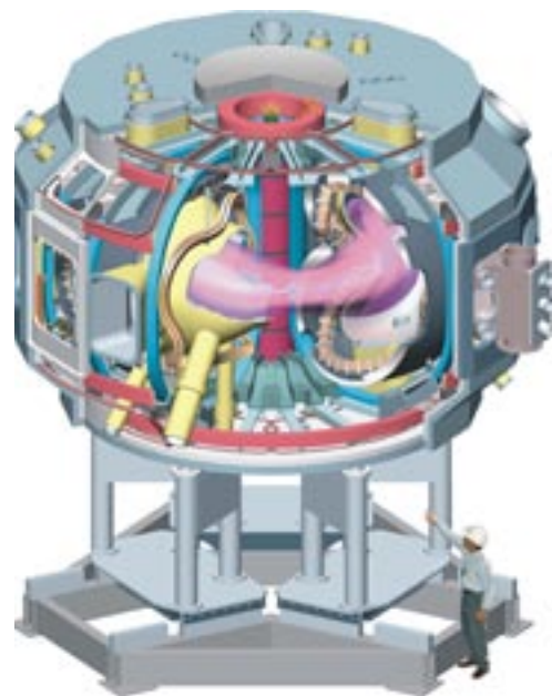
National Compact Stellarator Experiment
