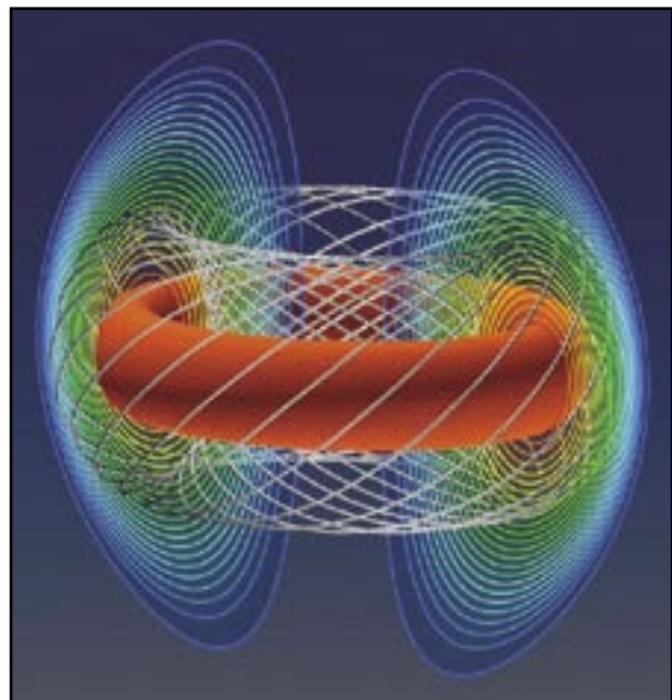
A three-dimensional nonlinear simulation of the National Spherical Torus Experiment using the M3D code.
