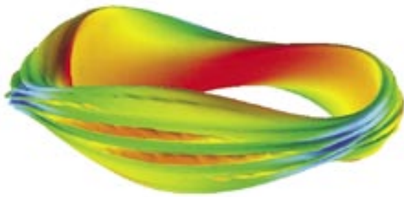
A three-dimensional simulation of a plasma in the National Compact Stellarator Experiment.
