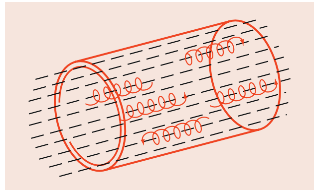
Motion of charged particles with magnetic field.
