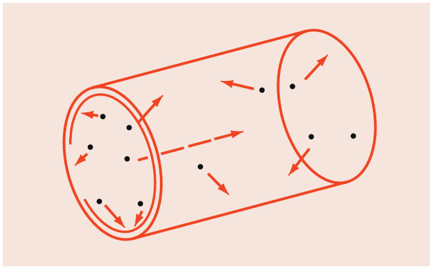
Motion of charged particles without magnetic field.
