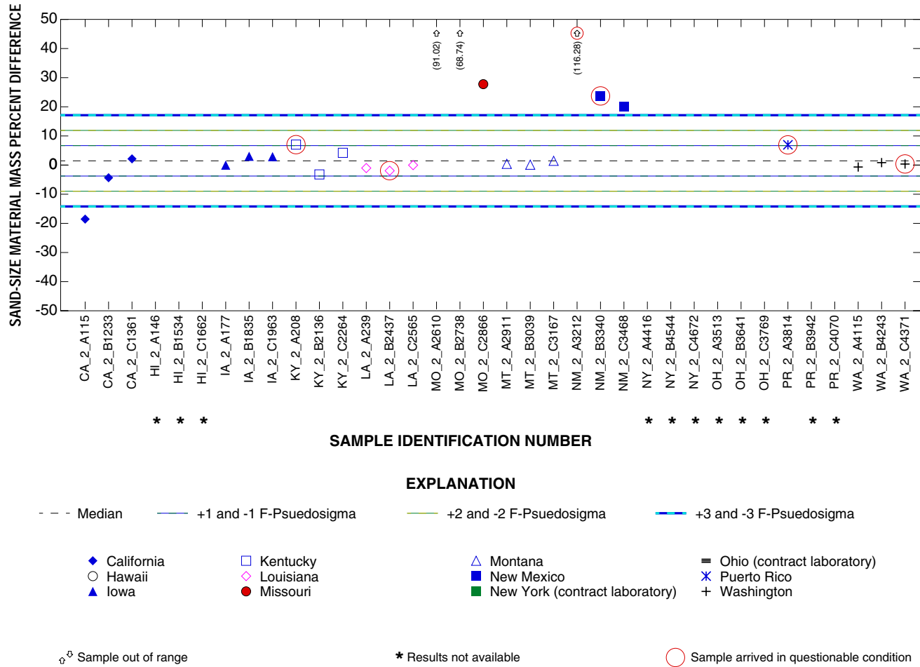
Figure 39. Sand-size material mass percent difference for samples containing 101 to 300 milligrams of fine-size material from study number 97-2, which was completed in September 1997.
