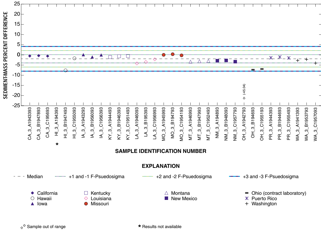
Figure 11. Sediment-mass percent difference for samples containing 2,200 to 3,200 milligrams of fine-size material from study number 96-1, which was completed in August 1996.
