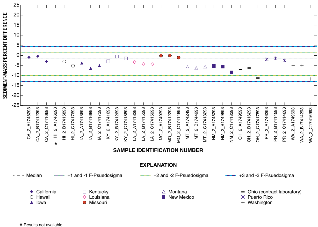
Figure 6. Sediment-mass percent difference for samples containing 101 to 300 milligrams of fine-size material from study number 96-1, which was completed in August 1996.
