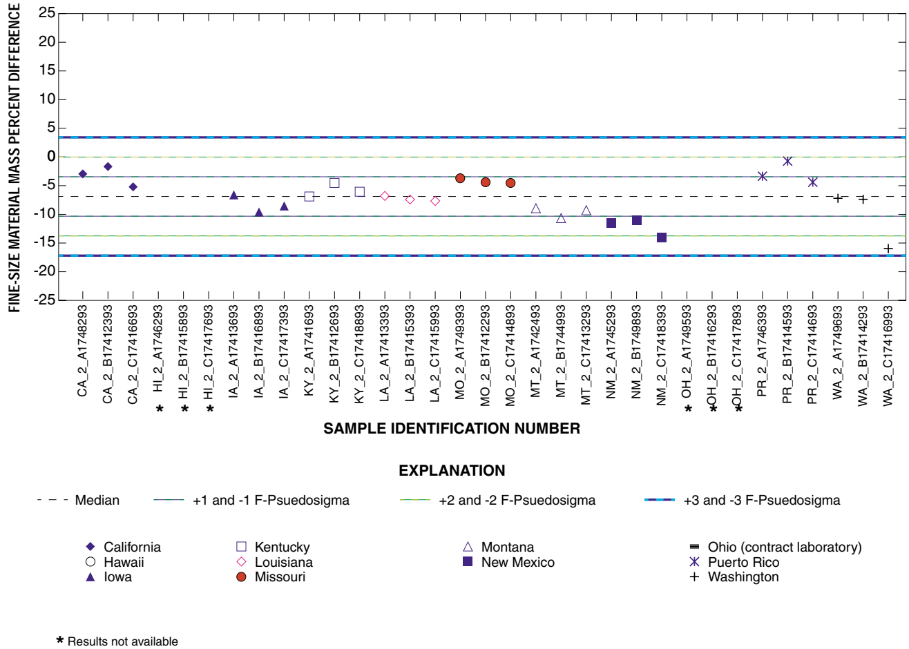
Figure 21. Fine-size material mass percent difference for samples containing 101 to 300 milligrams of fine-size material from study number 96-1, which was completed in August 1996.
