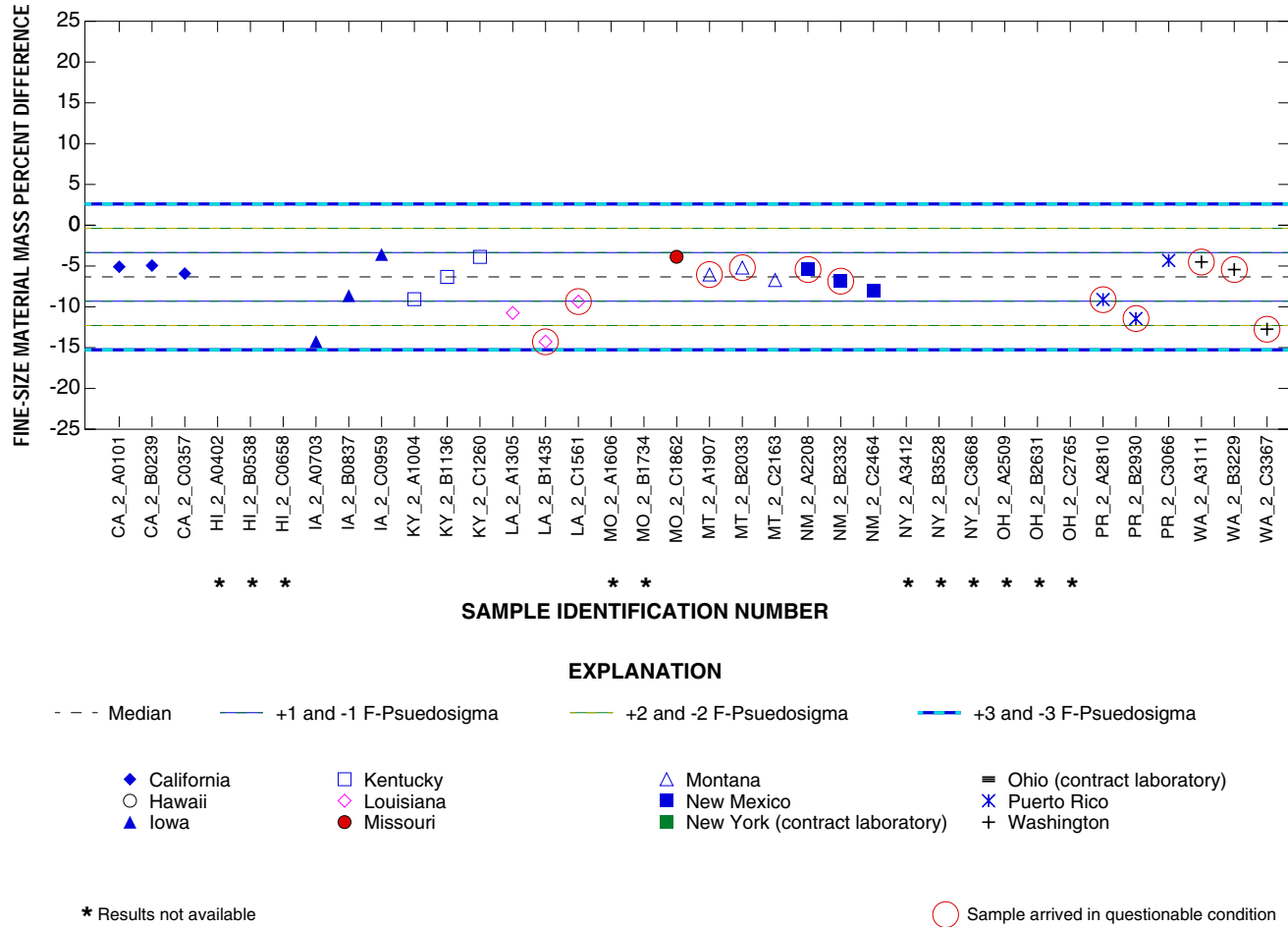
Figure 23. Fine-size material mass percent difference for samples containing 101 to 300 milligrams of fine-size material from study number 97-1, which was completed in July 1997.
