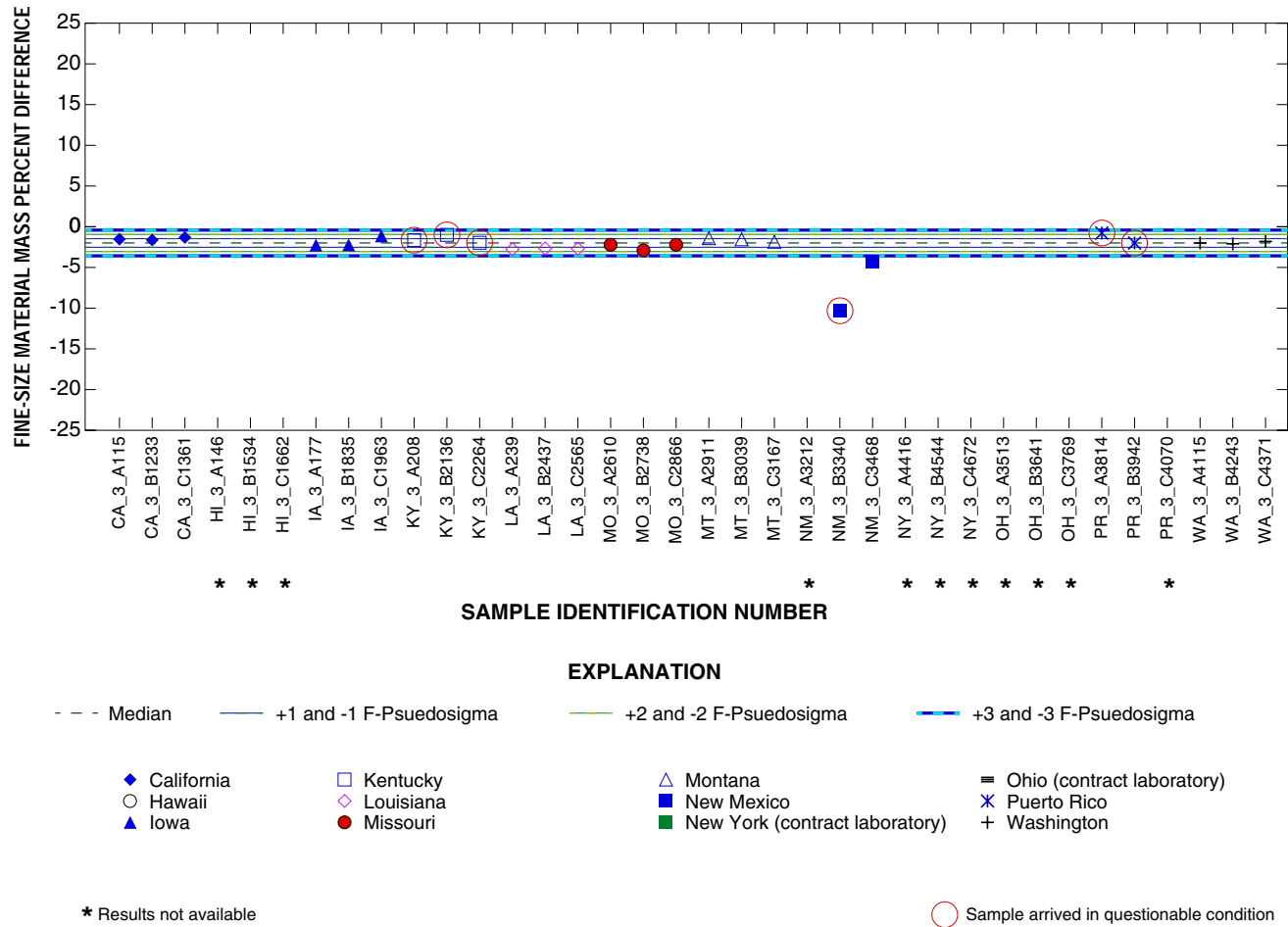
Figure 29. Fine-size material mass percent difference for samples containing 2,200 to 3,200 milligrams of fine-size material from study number 97-2, which was completed in September 1997.
