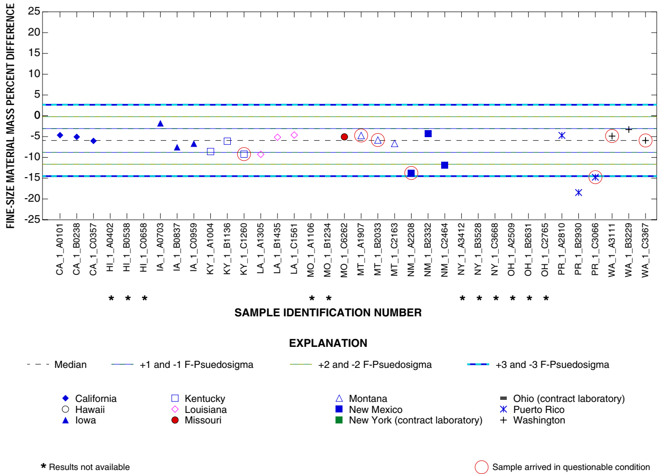
Figure 18. Fine-size material mass percent difference for samples containing 50 to 100 milligrams of fine-size material from study number 97-1, which was completed in July 1997.
