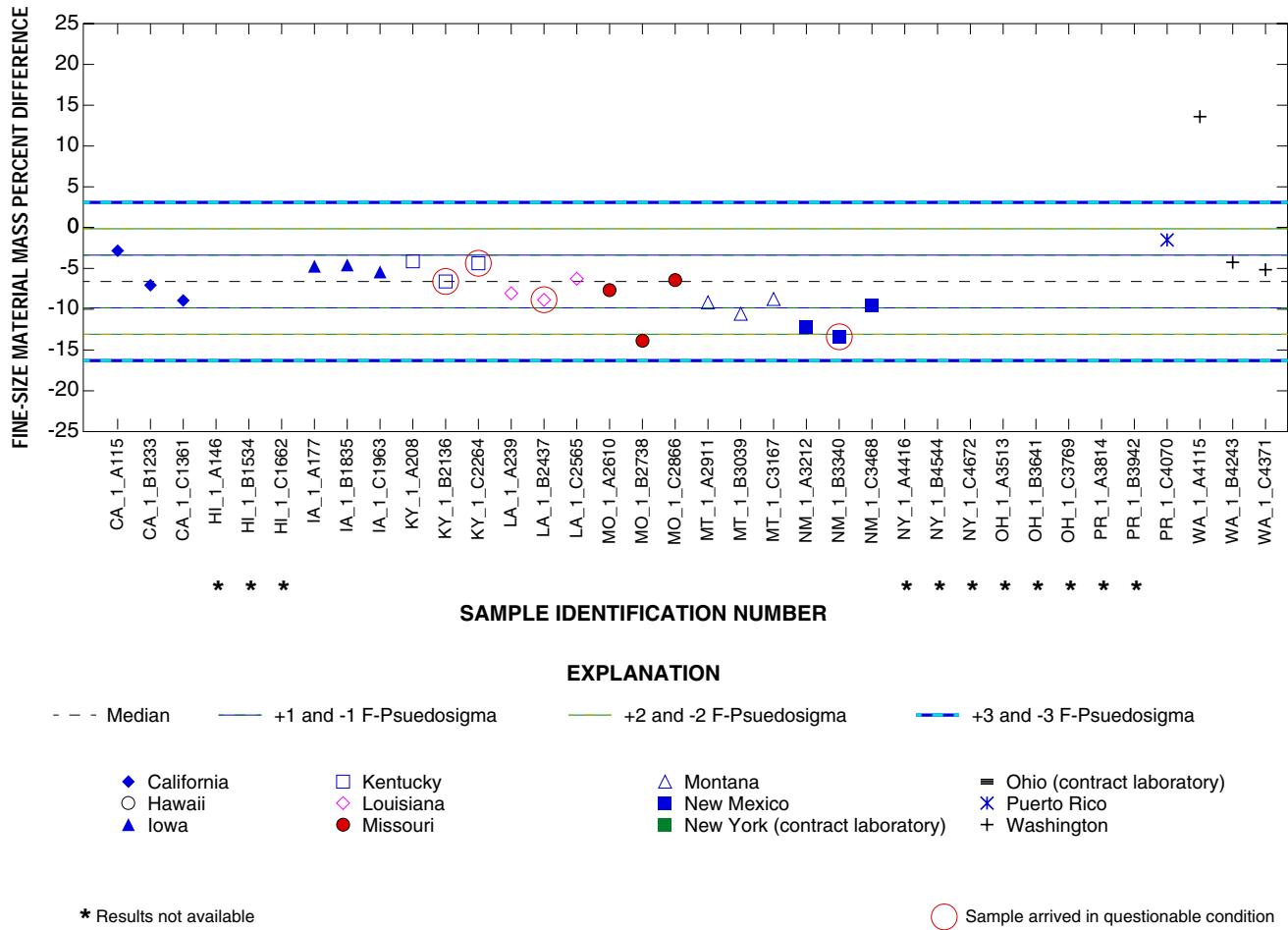
Figure 19. Fine-size material mass percent difference for samples containing 50 to 100 milligrams of fine-size material from study number 97-2, which was completed in September 1997.
