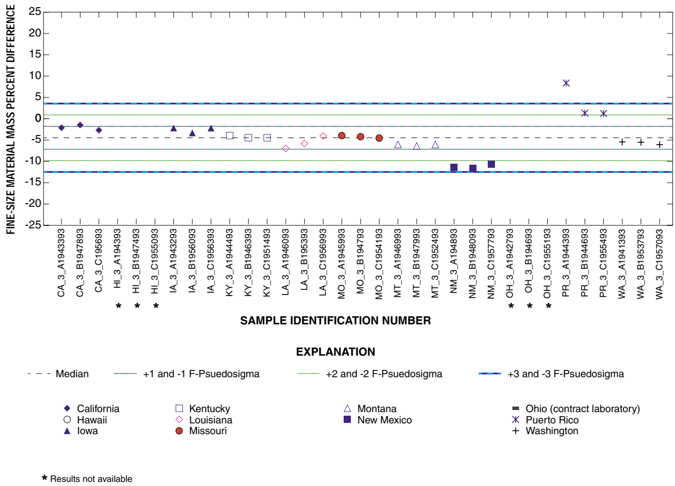
Figure 26. Fine-size material mass percent difference for samples containing 2,200 to 3,200 milligrams of fine-size material from study number 96-1, which was completed in August 1996.
