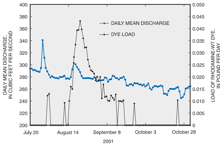
Figure 5. Daily mean discharge of Big Spring and estimated daily load of Rhodamine-WT dye in water discharging from Big Spring.
