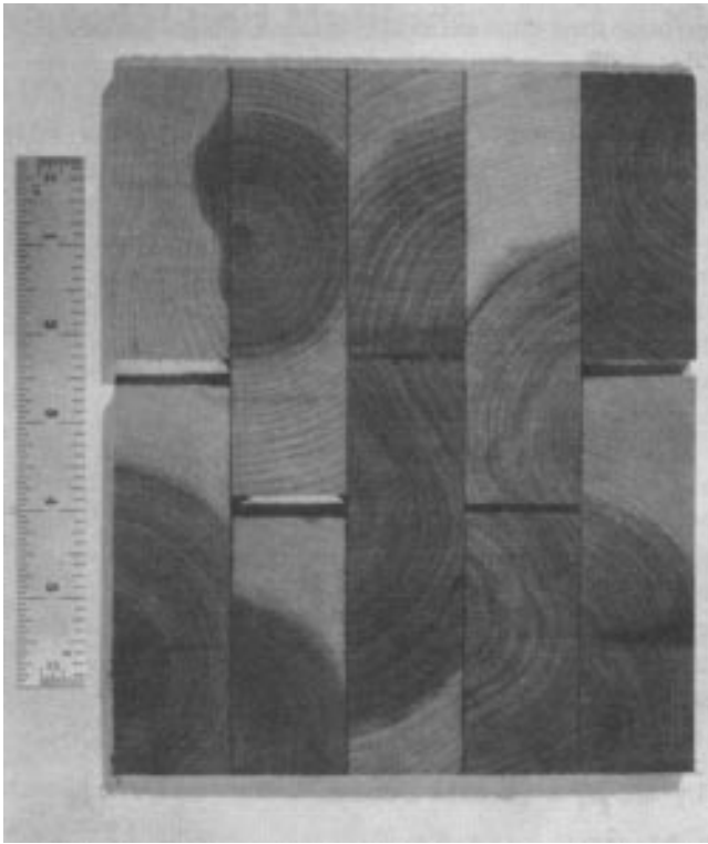
Figure 3—Cross section of 2 by 4/2 by 6 glulam combination, showing variation in gaps between edge joints.
