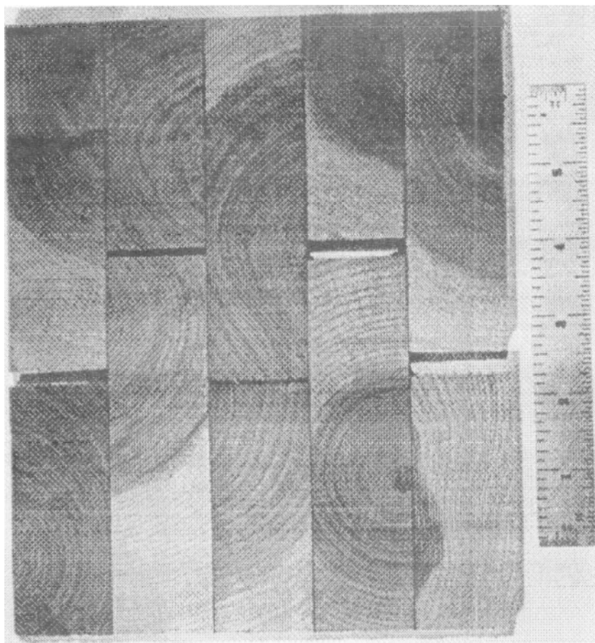
Figure 2. — Cross section of 2 by 4/2 by 6 glulam beam with glueline gaps.
