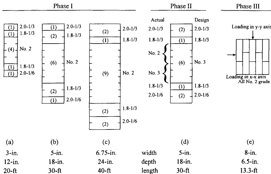
Figure 1. — Illustration of red maple glulam. Phase I beams (a-c) are 24F-1.8E combinations made from lumber sawn from whole trees. Phase II (d) is a 24F-18E combination made from lumber sawn from log cants. Phase III (e) is a wide-width combination made from cant-sawn 2 by 4 and 2 by 6 lumber.
