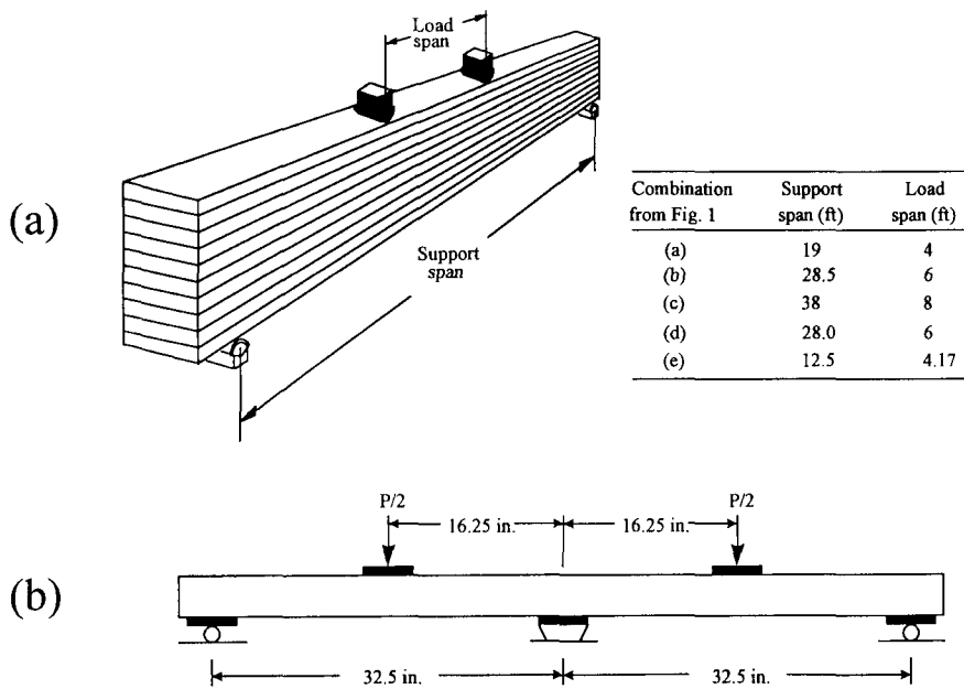
Figure 3. — Loading configurations for bending (a) and shear (b) tests of red maple glulam beams.
