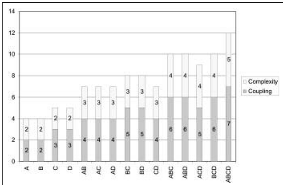
Figure 2: Metrics for Program Slices
