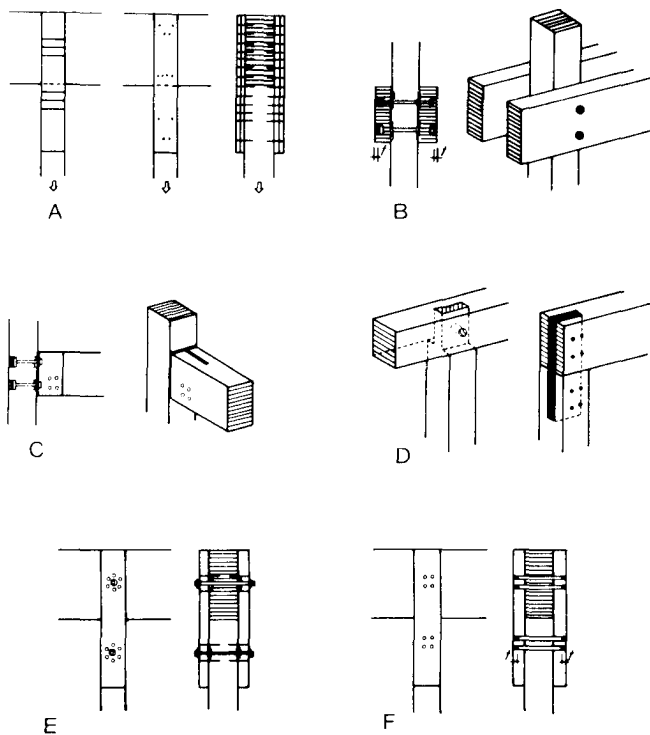
Figure 16.—Typical fire resistive timber connections recommended in Germany (23): A. Nailed butt-splice joint with sacrificial nailed cover plates. B. Split ring and bolted joint with countersunk and wood-capped bolt heads and nuts. C. Embedded steel shoe and bolted assembly with countersunk and wood-capped bolt heads. D. Simple embedded or wood-doweled connection. E. Split-ring connected butt-splice plate joint having exposed bolt head and nut but with cover plates nailed to members. F. Butt-splice joint employing embedded steel dowels and wood-capped holes. (M149 802)
