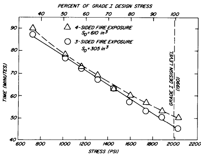
Figure 12.—Influence of applied stress level on fire endurance of glulam beams exposed to fire on three and four sides. (Three-sided beam section modulus = 305 in. 3 , four-sided beam section modulus = 610 in. 3 .) (M149 245)
