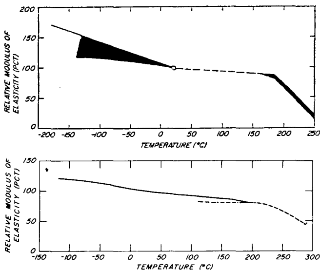
Figure 3.—Effect of temperature on E parallel to grain at near 0 percent MC and at about 12 percent MC. E is 100 percent at 20° C. Banded areas indicate variability in results reported by various researchers (17). A. Moisture content of 12 percent. B. Moisture content of 0 percent. (M148 689) (M149 818)
