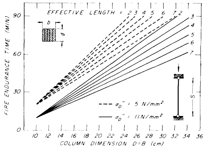
Figure 14.—Square laminated wood column fire endurance time as function of column dimension (modified from Haksever and Meyer-Ottens (20)). (1 N/mm 2 = 145.04 lb/in. 2 ) (M149 819)
