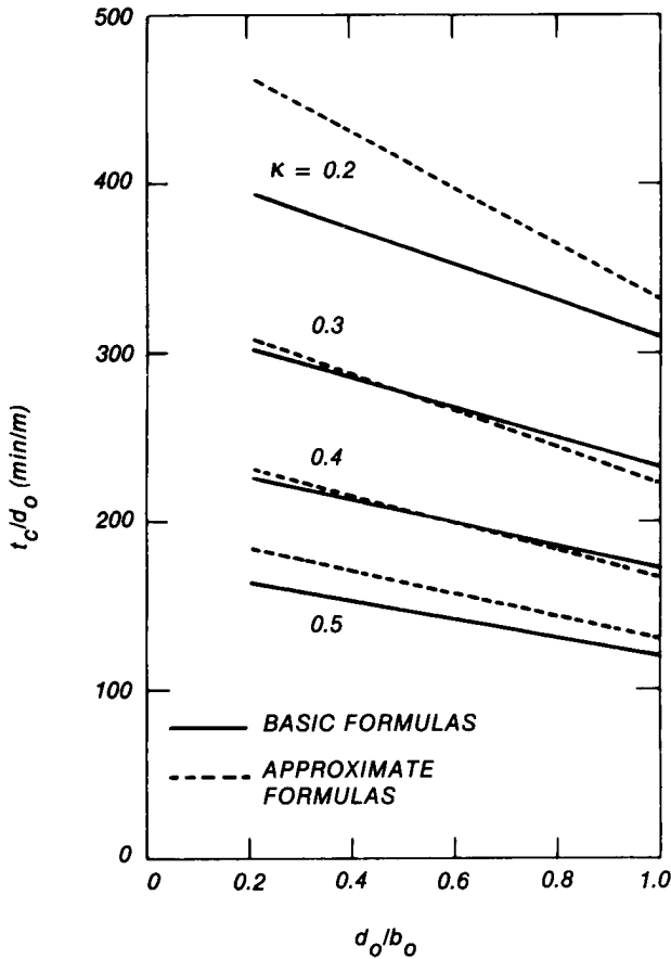
Figure 13.—Fire endurance of columns fire exposed on all four sides as a function of size (m) and load (31). (M149 813)
