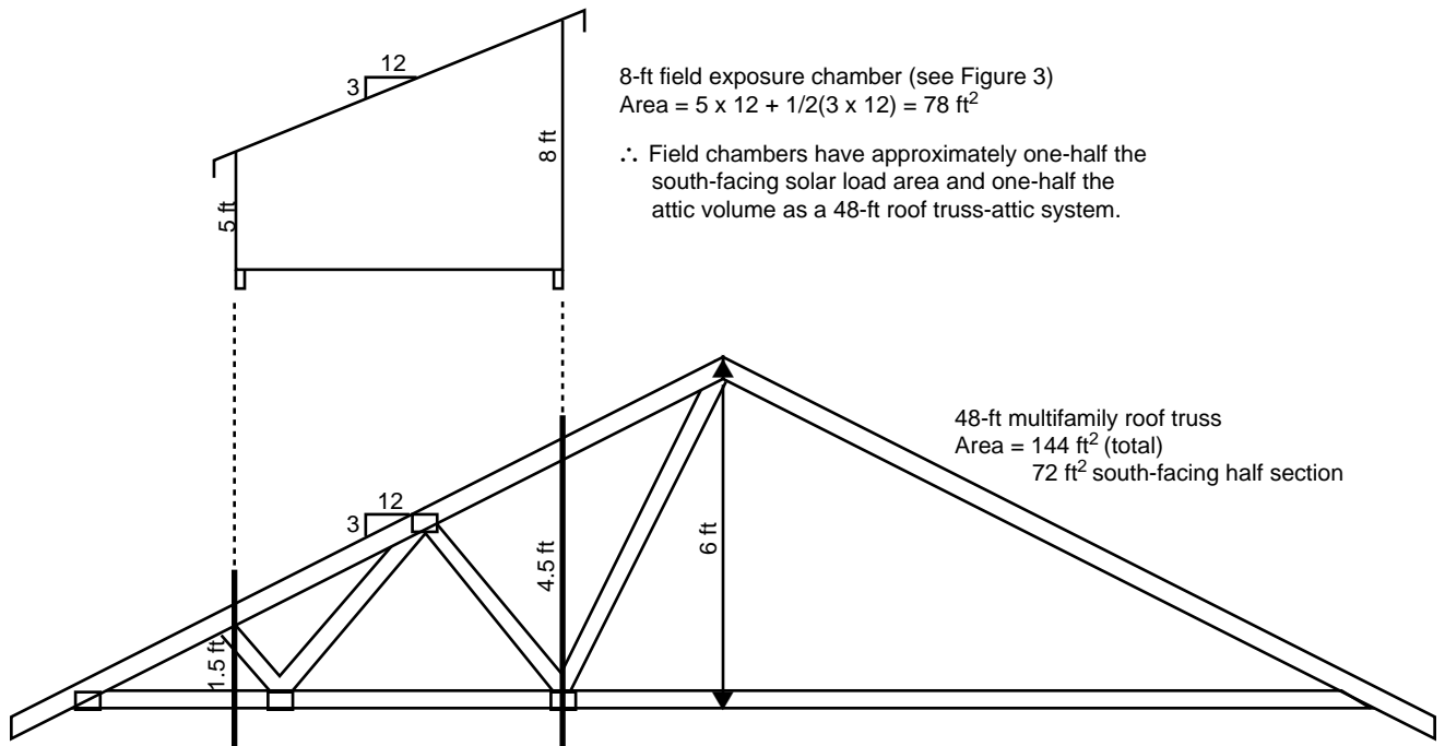
Figure 2—View of field exposure chamber in relation to roof truss of multifamily structure. Field chamber has approximately half the south-facing solar load area and half the attic volume as that of a 48-ft (14.6-m) roof truss-attic system. 1 \text{ ft}^2 = 0.09 \text{ m}^2 .
