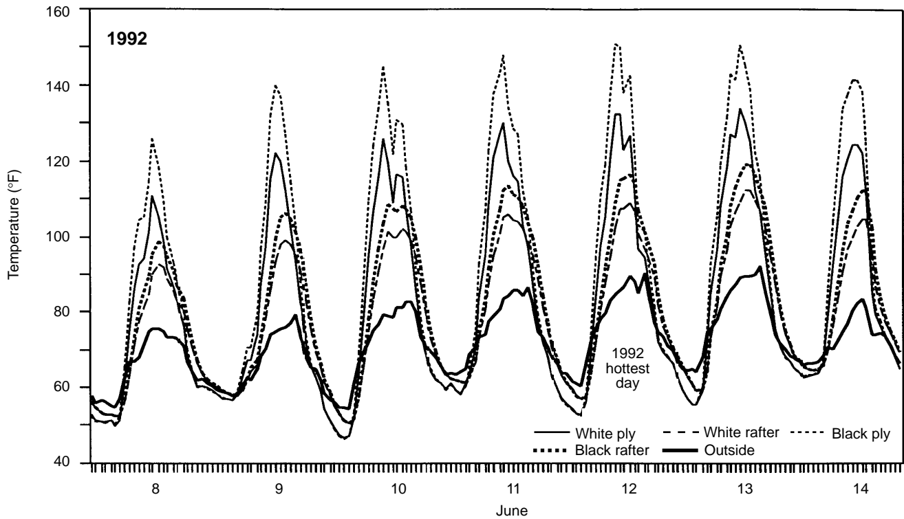
Figure 14—Comparison of temperature histories in specified locations in black- and white-shingled exposure chambers in 1992.
