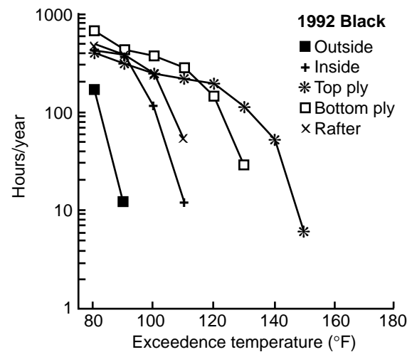
Figure 6—Number of hours that recorded temperatures at specified locations went beyond the exceedence temperature in black-shingled exposure chamber in 1992. Exceedence temperature is the range between some minimum temperature limit and next higher exceedence temperature limit. Outside and inside refer to exterior and interior temperatures of exposure chamber. Top plywood and bottom ply refer to temperatures of plywood sheathing at respective places. ^{\circ}T_C = (T_F - 32)/1.8 .
