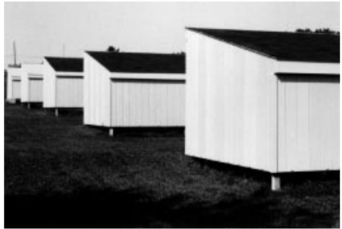
Figure 1—Outdoor field exposure chambers built near Madison, Wisconsin (latitude = 43.4° north). Each chamber holds 96 field exposure specimens. (M95 0057–24A)
