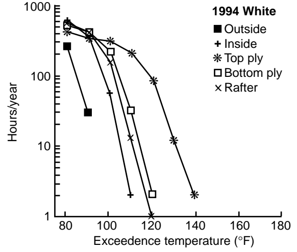
Figure 11—Number of hours that recorded temperatures at specified locations went beyond the exceedence temperature in white-shingled exposure chamber in 1994.
