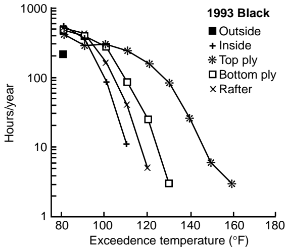
Figure 8—Number of hours that recorded temperatures at specified locations went beyond the exceedence temperature in black-shingled exposure chamber in 1993.
