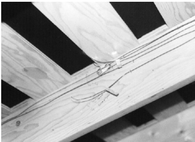
Figure 4—Placement detail of thermocouples for monitoring temperatures inside field exposure chamber and openings in sheathing plywood intended to accept sample specimens. All data were recorded with field exposure specimens in place. (M95 0057–22A)
