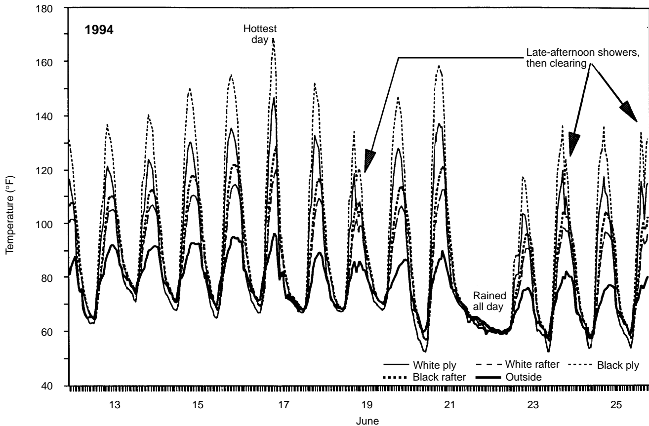
Figure 15—Comparison of temperature histories in specified locations in black- and white-shingled exposure chambers in 1994.
