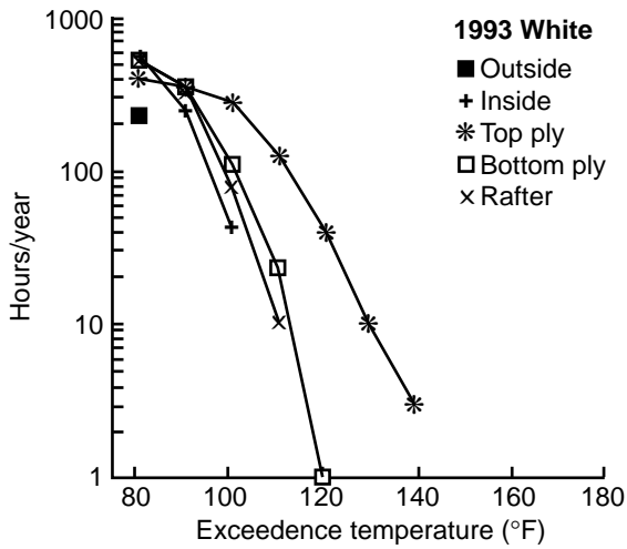
Figure 9—Number of hours that recorded temperatures at specified locations went beyond the exceedence temperature in white-shingled exposure chamber in 1993.
