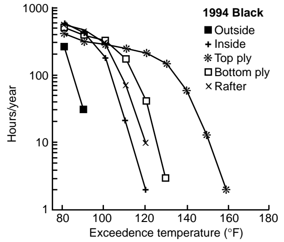
Figure 10—Number of hours that recorded temperatures at specified locations went beyond the exceedence temperature in black-shingled exposure chamber in 1994.
