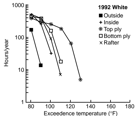
Figure 7—Number of hours that recorded temperatures at specified locations went beyond the exceedence temperature in white-shingled exposure chamber in 1992.
