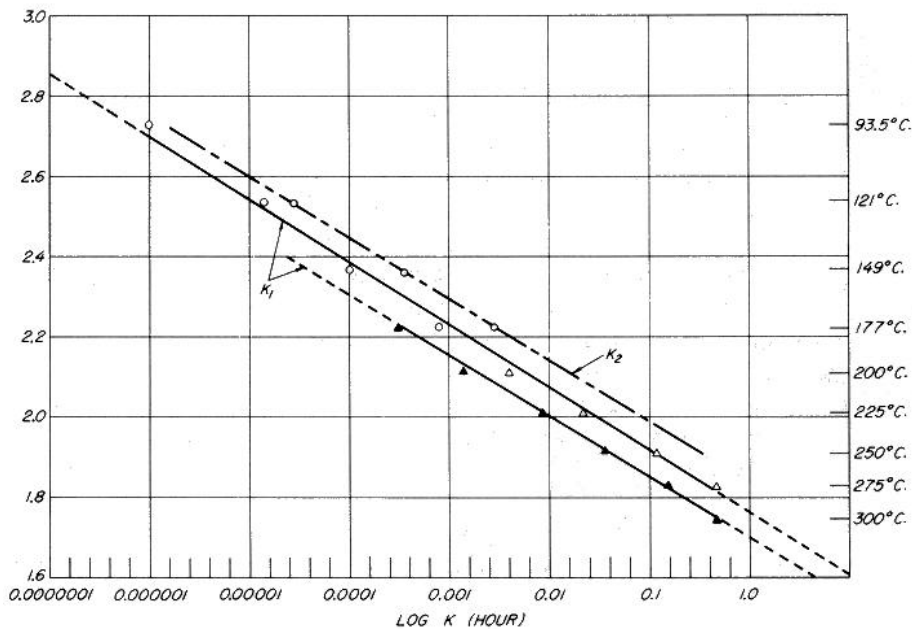
Figure 1. Reciprocal of absolute temperature versus logarithm of K , where K , the reaction constant, is determined from weight loss/time experiments for heated wood samples. Open symbols for specimens heated in oven. Shaded symbols for specimens heated beneath the surface of a molten metal.
