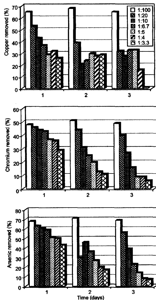
Fig. 1. Percentage copper, chromium, and arsenic removed during three sequential 24-h extractions reusing oxalic acid solutions at various ratios (v/w) to fresh CCA-treated particles.
