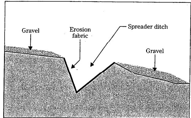
Detailed cross-section of level spreader trench for dispersing runoff along the contour
