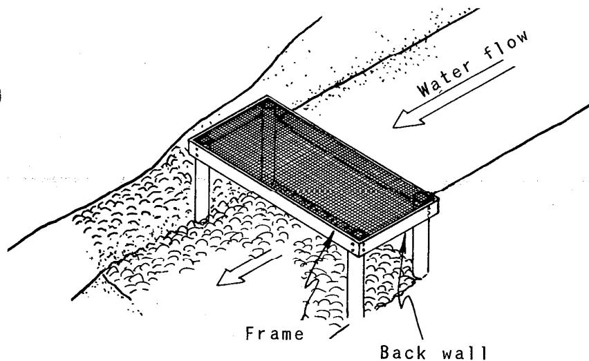
A screened overfall in the emergency spillway helps keep unwanted fish from entering the pond.
