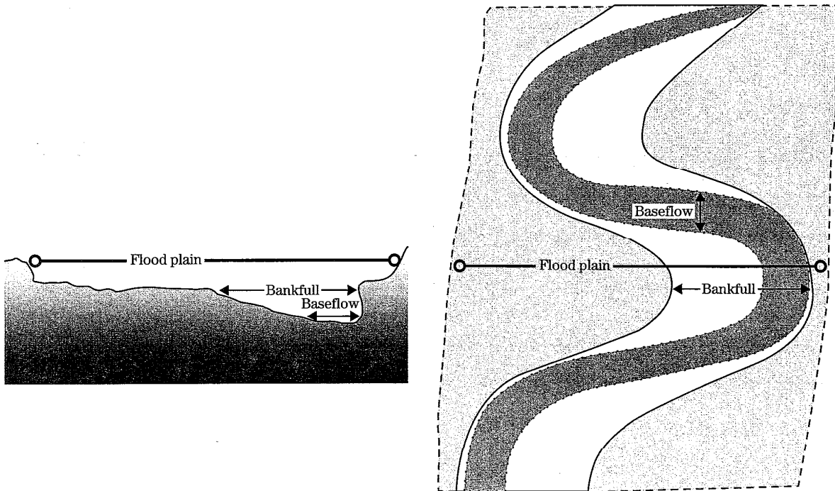
Figure 3 Baseflow, bankfull, and flood plain locations (Rosgen 1996)
