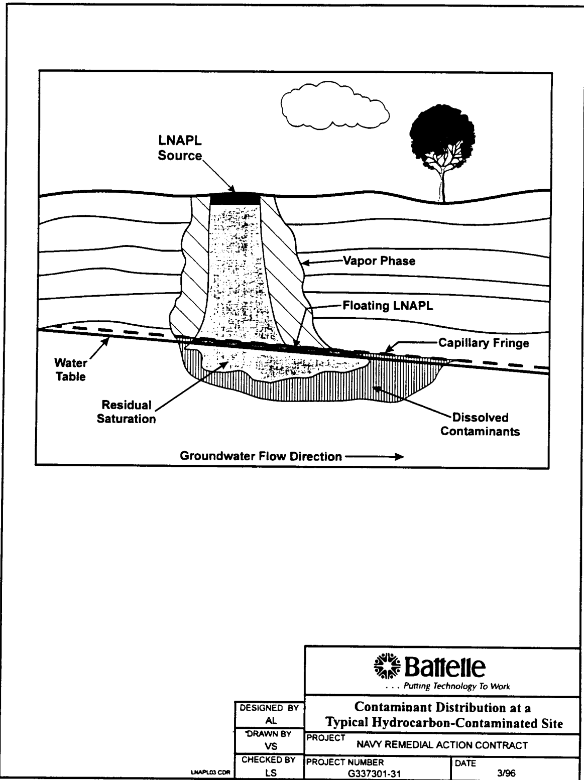
Figure 2. Contaminant Distribution at a Typical Hydrocarbon-Contaminated Site.
