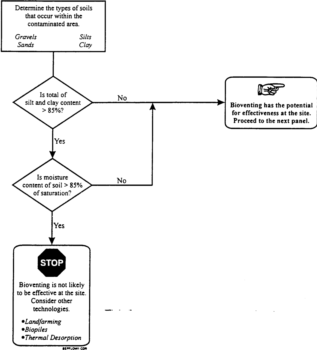
Figure 3. Bioventing Evaluation Process Flowchart.
