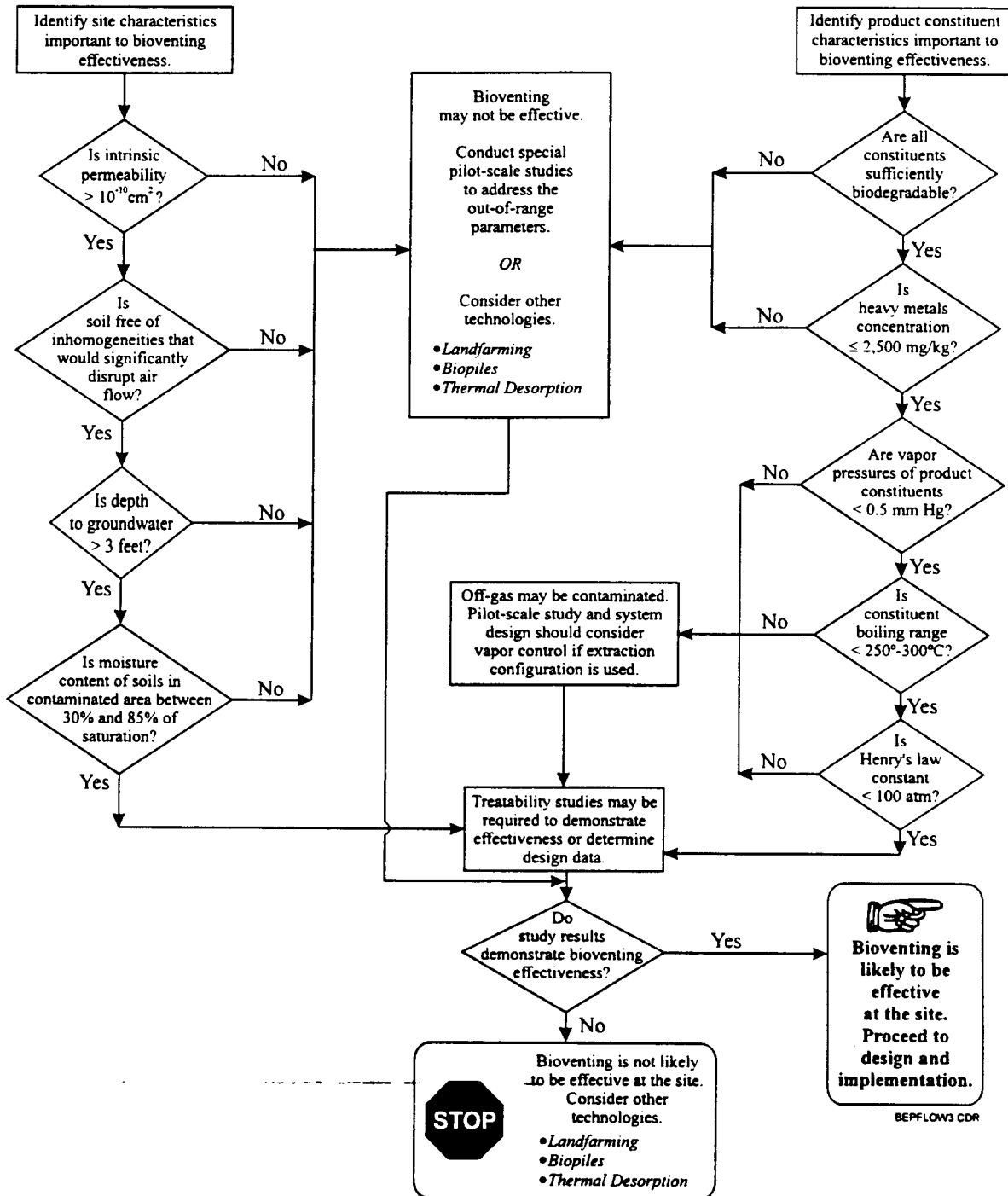
Figure 3. Bioventing Evaluation Process Flowchart (continued).
