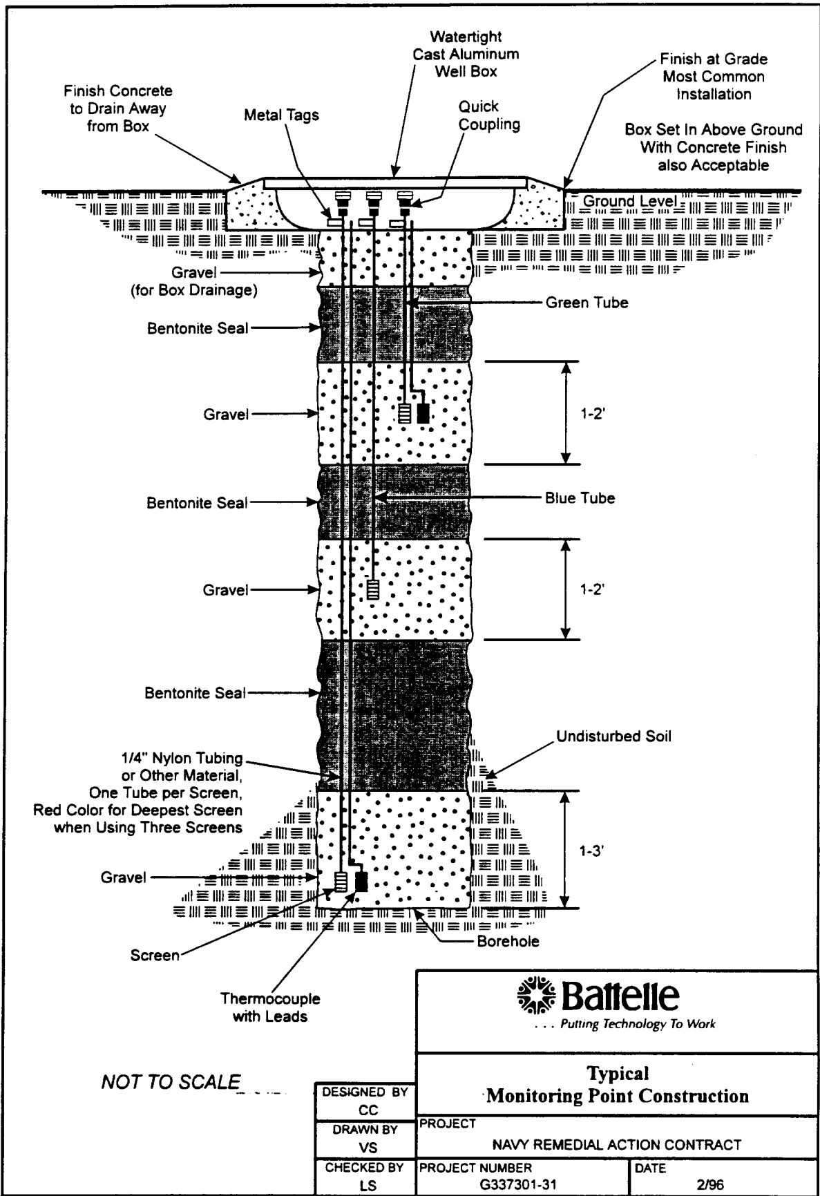
Figure 5. Illustration of a Typical Monitoring Point for Bioventing.
