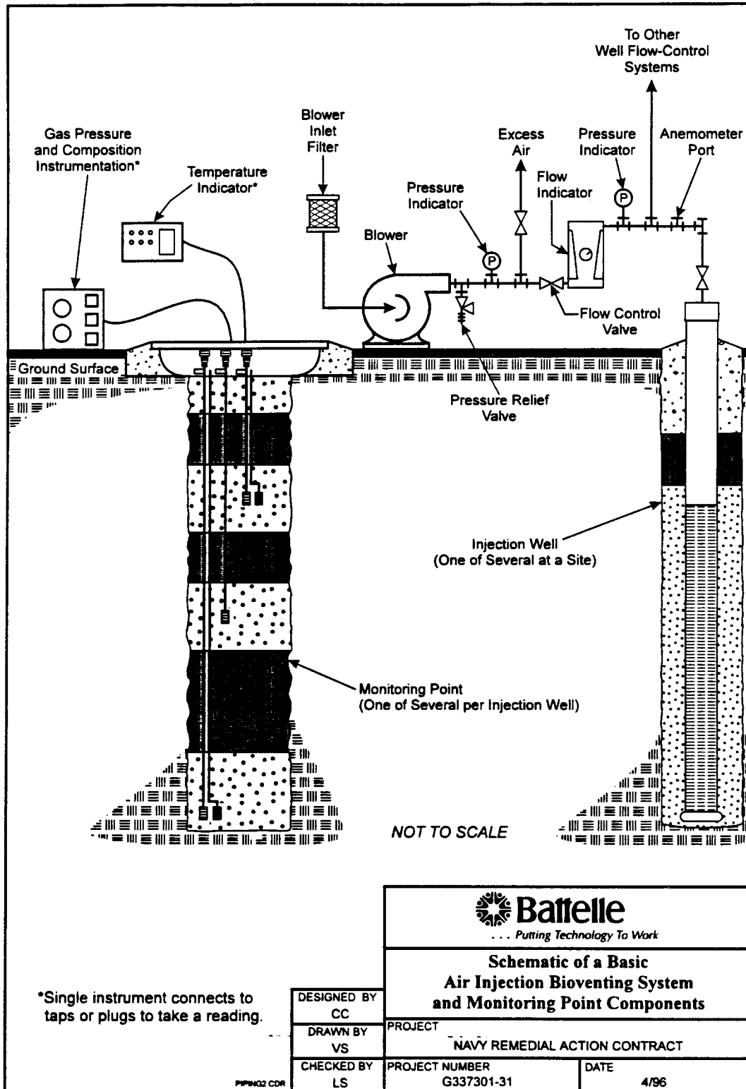
Figure 1. Schematic of a Basic Air Injection Bioventing System and Monitoring Point Components.
