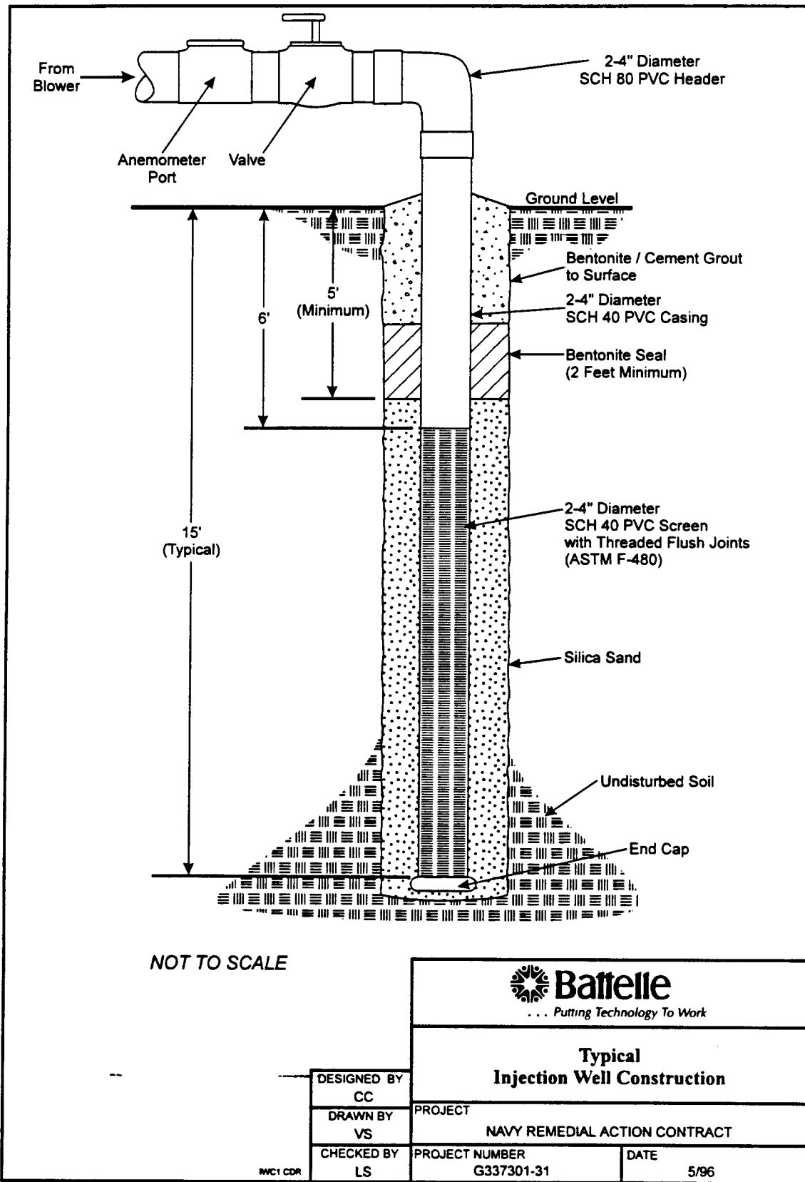
Figure 4. Illustration of a Typical Vent Well for Bioventing.
