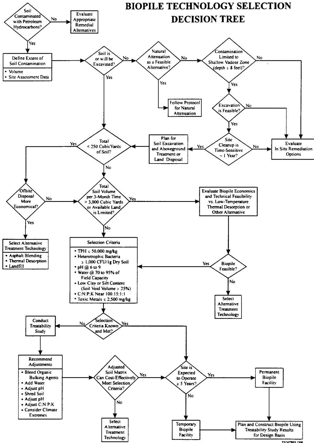
Figure 1. Biopile Technology Selection Decision Tree.
