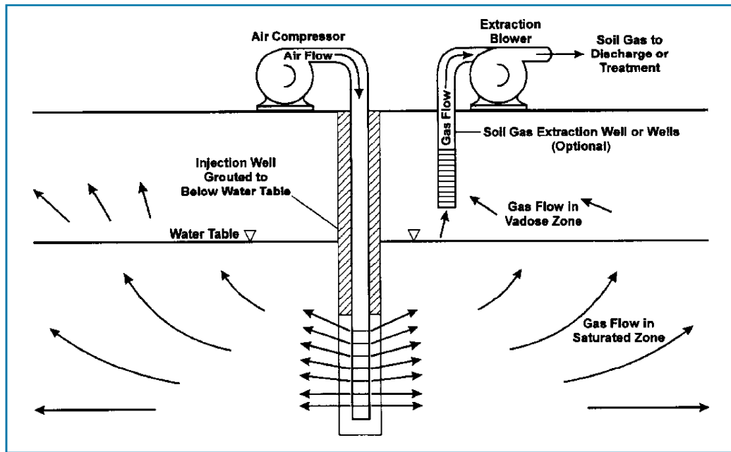
Figure 1. In-situ air sparging system.
