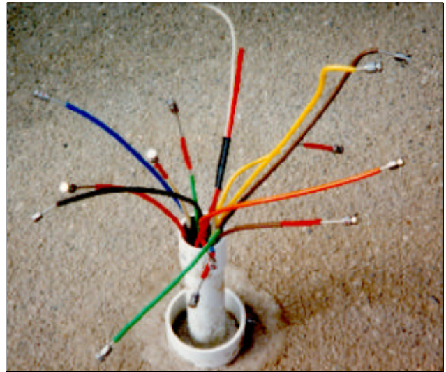
Figure 4. Miniaturized in-situ pressure sensors.
