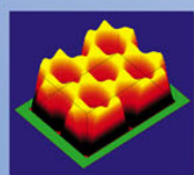
Magnesium Diboride
