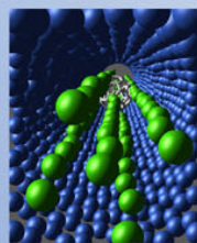
Buckyball Piston
