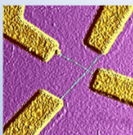
Single-walled Nanotubes
