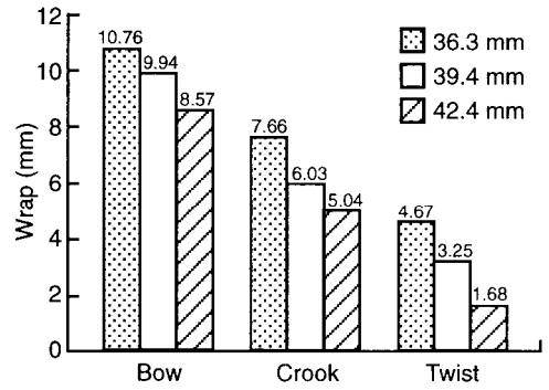
FIG. 6. Effect of board thickness on crook, bow, and twist in experimental groups 3o and 3r
