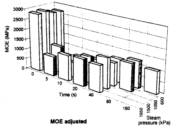
FIG. 13. Adjusted MOE.
