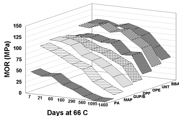
Measured Loss in MOR at 66 C
