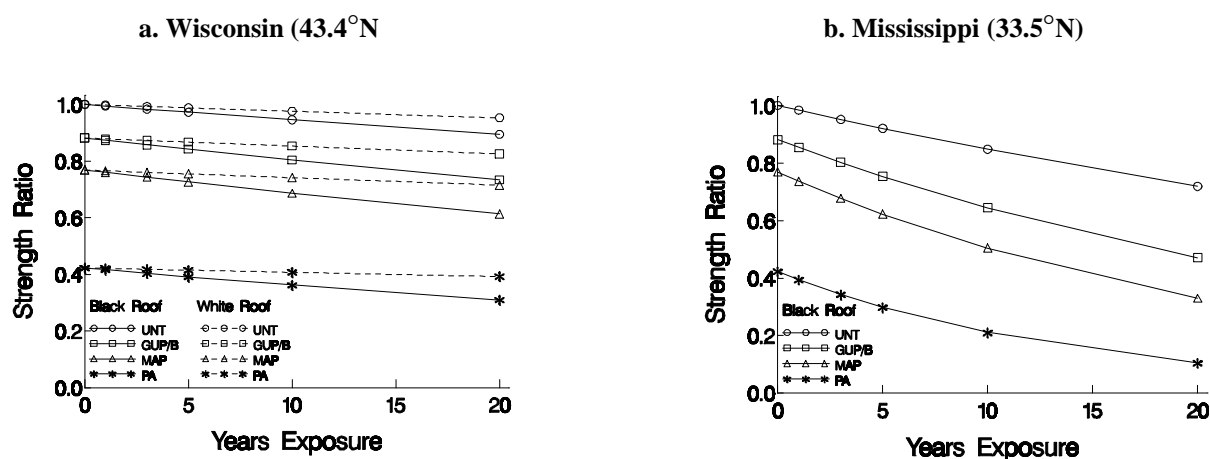
Figure 9. Predicted plywood strength after 20 years of in-service exposure using a preliminary residual serviceability prediction model. Each treatment has progressively lower pH (in the order of GUP/B, MAP, PA) (J.F. Murphy, P.K. Lebow, J.E. Winandy, Development of residual service-life models for plywood roof sheathing (unpublished)) (UNT untreated, GUP/B guanylurea phosphate/boric acid, MAP monoammonium phosphate, PA phosphoric acid).
