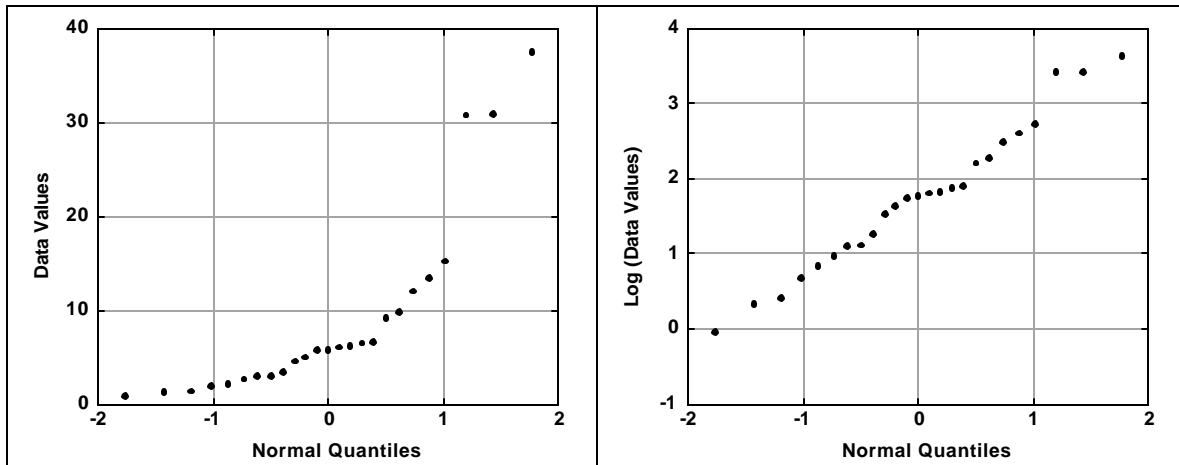
Fig. 2.5-8. Normal and Log-Normal Probability Plots of Log-Normal Data
