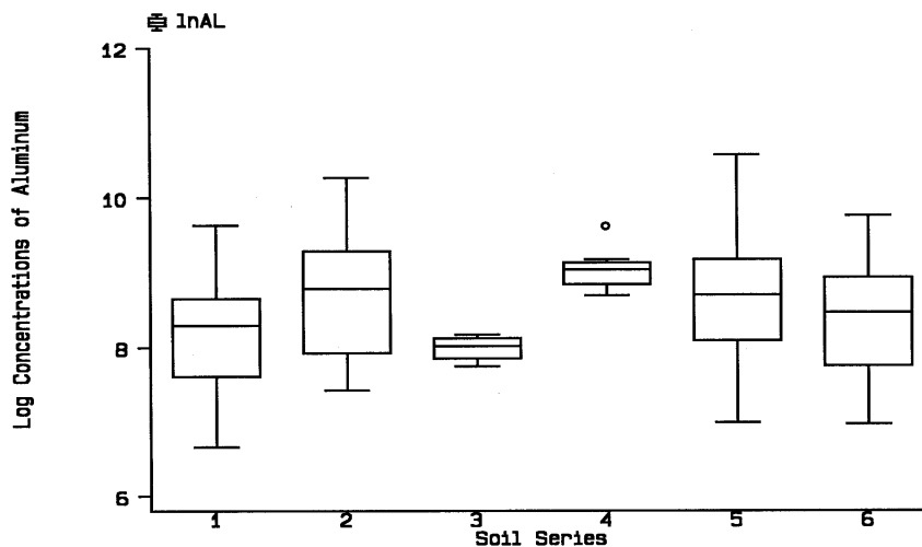
Fig. 2.5-9. Boxplots of Log-transformed Aluminum Concentrations in Six Different Soil Series
