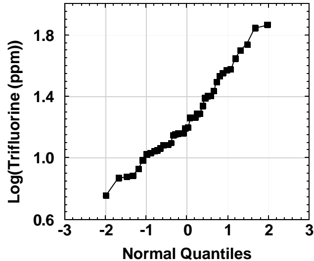
Figure 2.5-7. Example of a Probability Plot to Test that the Data have a Lognormal Distribution
