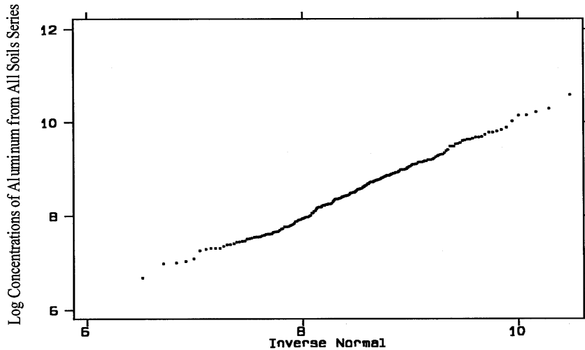
Fig. 2.5-10. Normal Probability Plot of Log-Transformed Aluminum Data from All Soil Series
