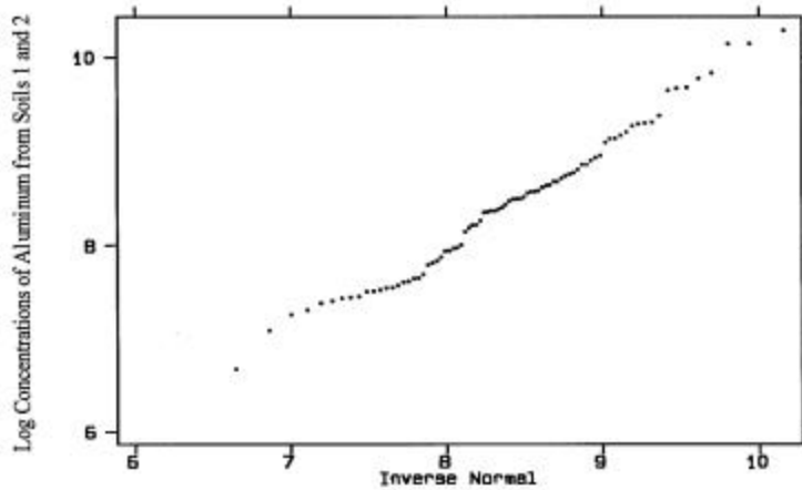
Figure 2.5-11. Normal Probability Plot of Log-Transformed Aluminum Data from the Combined Soil Series 1 and 2
