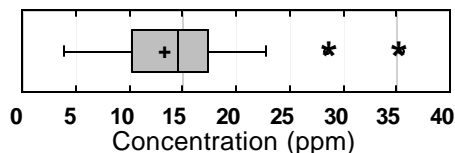
Figure 2.5-3. Example: Boxplot (Box-and-Whisker Plot).
