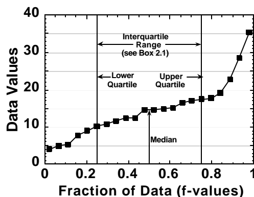
Figure 2.5-4. Example: Quantile Plot of a Skewed Data Set
