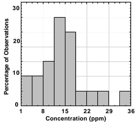
Figure 2.5-2. Histogram with Smaller Interval Widths
