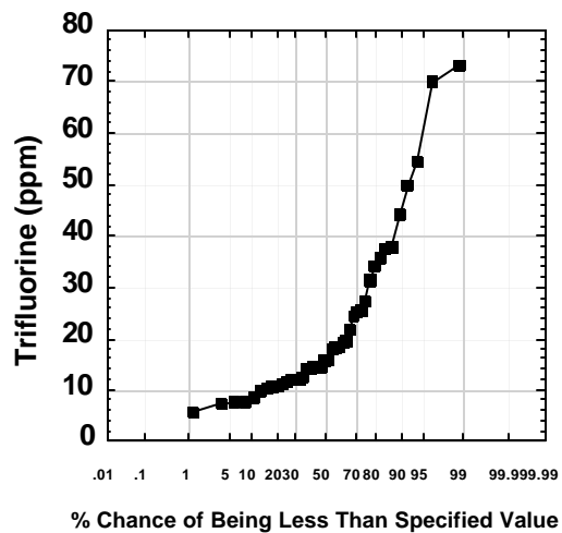
Figure 2.5-6. Example: Probability Plot for Normal Hypothesized Distribution (100 x Probability on the x-Axis).
