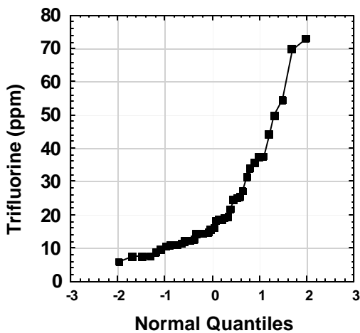
Figure 2.5-5. Example: Probability Plot for Which the Hypothesized Distribution is Normal (Quantiles on the x-Axis).
