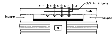
Curb Splice Detail Side View
