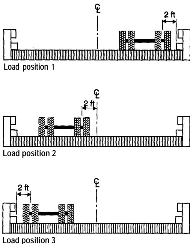
Figure 14 - Transverse load positions used for Load Test 1. Vehicles in the right lane face North, into the page; those in the left lane face South, out of the page. For all load positions, the longitudinal centroid of the vehicle was placed over the bridge centerspan.
