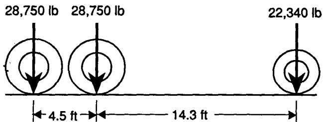
Figure 13—Load Test 1 vehicle configuration and axle loads. The transverse vehicle track width was 6 ft, measured center-to-center of the rear tires.
